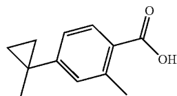
2-Methyl-4-(1-methyl-cyclopropyl)-benzoic acid
