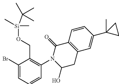
2-[3-Bromo-2-(tert-butyl-dimethyl-silanyloxymethyl)-phenyl]-3-hydroxy-7-(1-methyl-cyclopropyl)-3,4-dihydro-2H-isoquinolin-1-one
