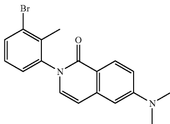
2-(3-Bromo-2-methyl-phenyl)-6-dimethylamino-2H-isoquinolin-1-one
