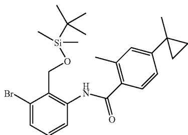
N-[3-Bromo-2-(tert-butyl-dimethyl-silanyloxymethyl)-phenyl]-2-methyl-4-(1-methyl-cyclopropyl)-benzamide
