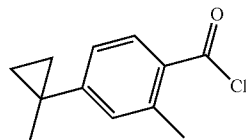
2-Methyl-4-(1-methyl-cyclopropyl)-benzoyl chloride
