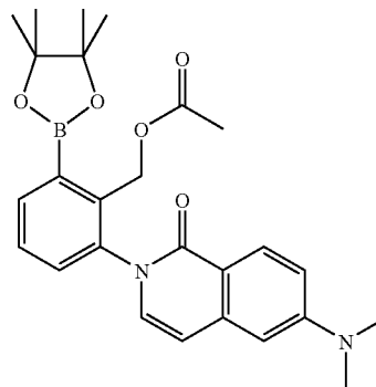
Acetic acid 2-(6-dimethylamino-1-oxo-1H-isoquinolin-2-yl)-6-(4,4,5,5-tetramethyl-[1,3,2]dioxaborolan-2-yl)-benzyl ester
