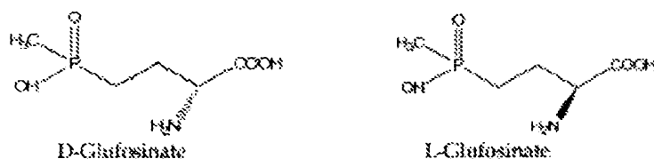
Fig. 1. Chemical structures of D-glufosinate and L-glufosinate.
