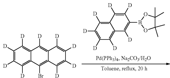
Intermediate 4L:
