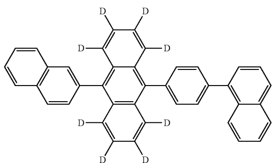
Compound H12:
