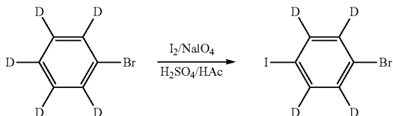
Intermediate 4B:
