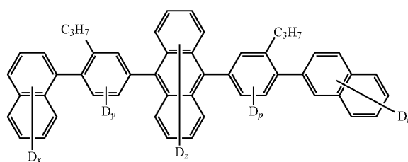
Compound H7:
