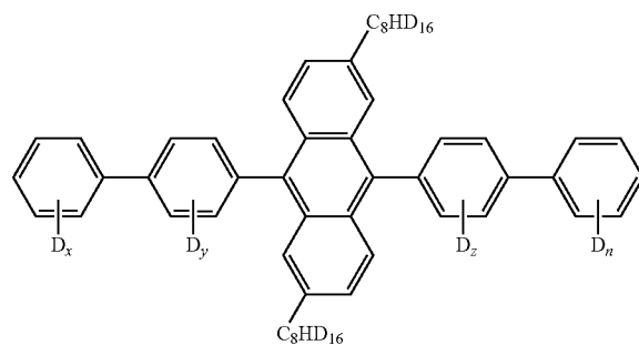
Compound H6:
