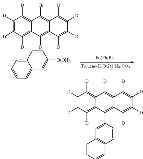
Intermediate 4J:
