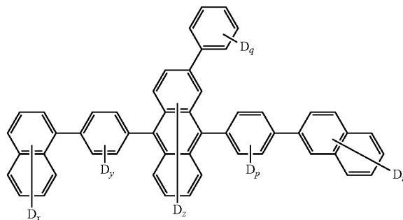
Compound H5:
