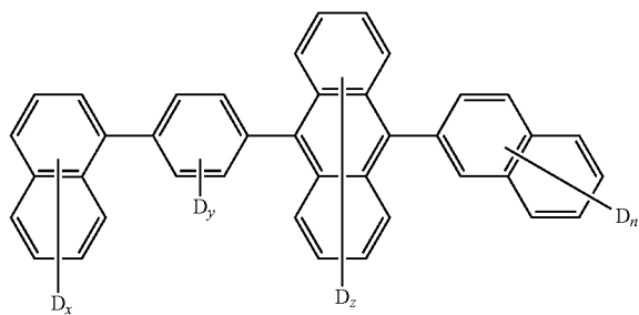
Compound H1:
