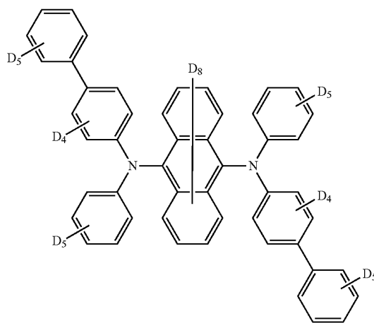
Compound E2:
