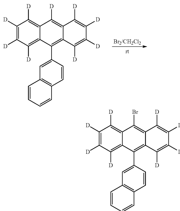
Intermediate 4K:
