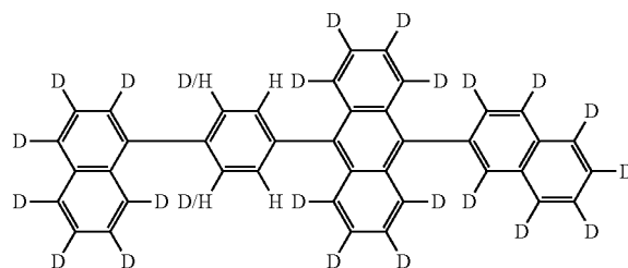
Compound H14:
