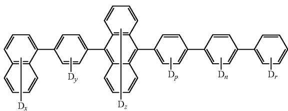
Compound H3:
