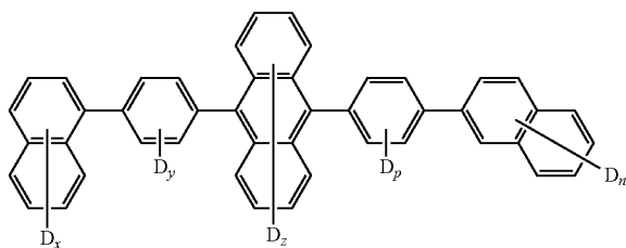
Compound H2:
