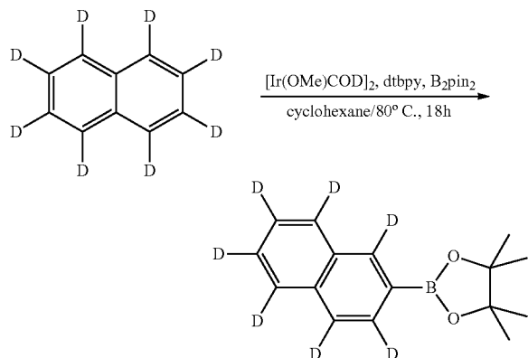
Intermediate 4I:
