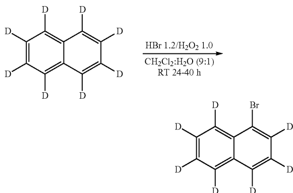
Intermediate 4E:
