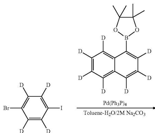
Intermediate 4E:
