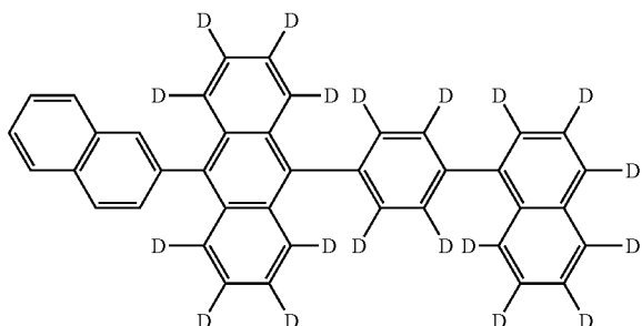
Compound H10:
