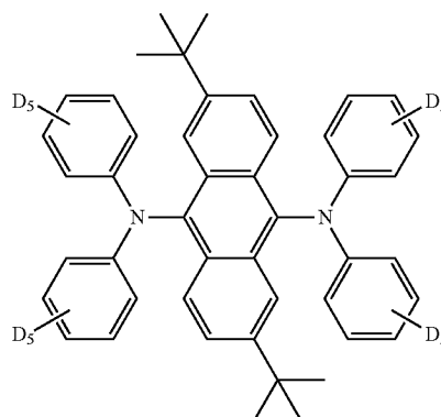
Compound E1:
