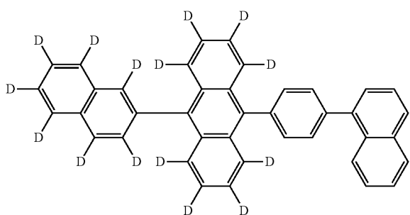
Compound H11:
