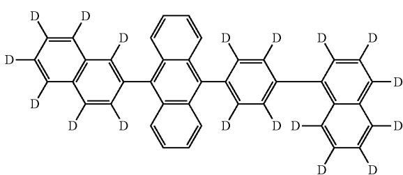
Compound H13:
