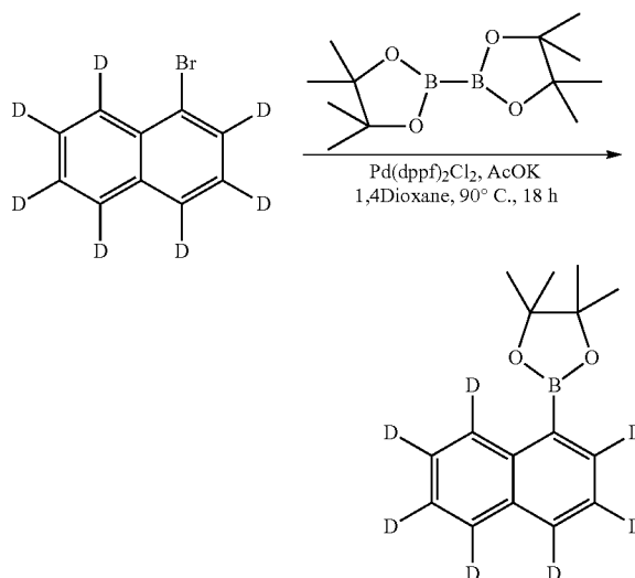
Intermediate 4D:
