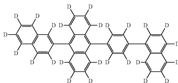
Compound H8:
