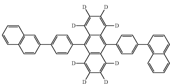
Compound H13:
