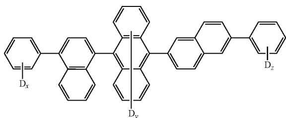
Compound H4:
