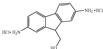
9-hydroxymethyl-2,7-diaminofluorene dihydrochloride
