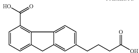
7-(3-carboxy-propyl)-4-fluorencarboxylic acid
