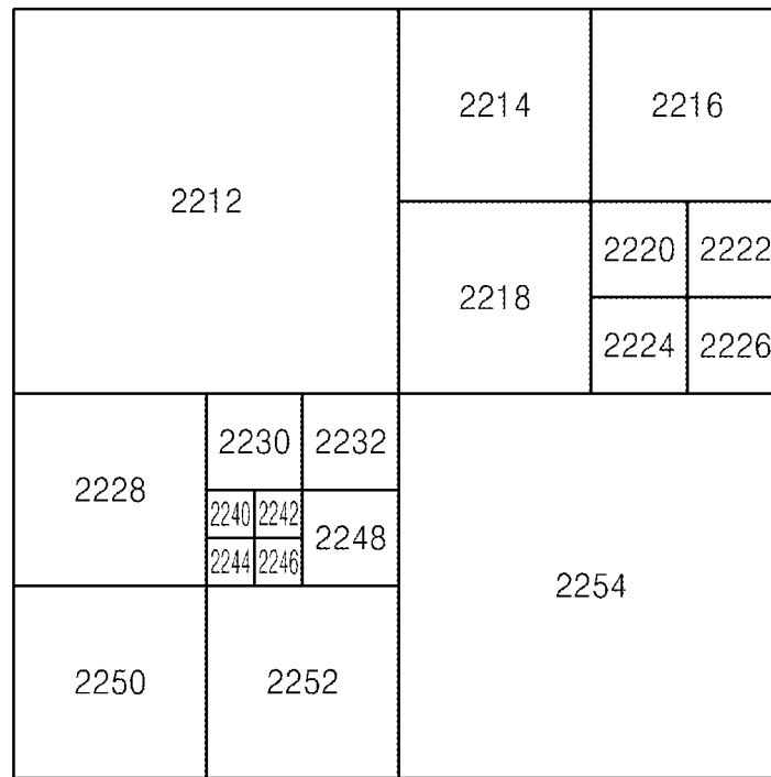
CODING UNIT (2210)
