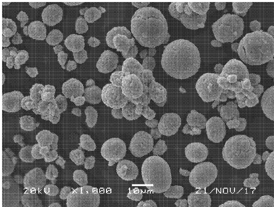
Fig. 3(b) NMC622 coated by \text{Li}_3\text{AlO}_{2.85}\text{F}_{0.3} (Al:F:Al-O = 5:95 mol/mol)
