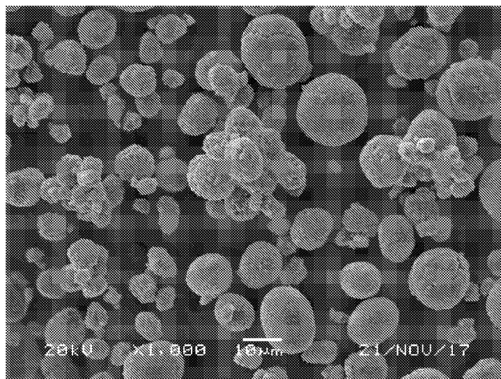
Fig. 3(b) NMC622 coated by Li 3 AlO 2.85 F 0.3 (Al:F:Al-O = 5:95 mol/mol)
