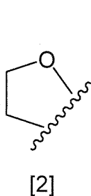
[Chemical Formula 2]
