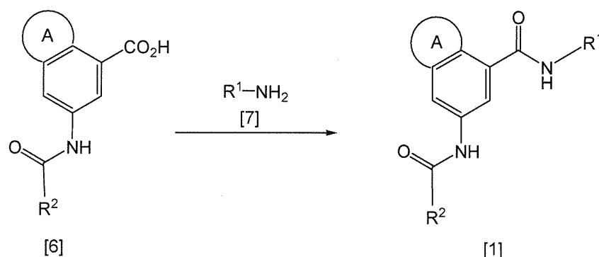
[Formula 4]
