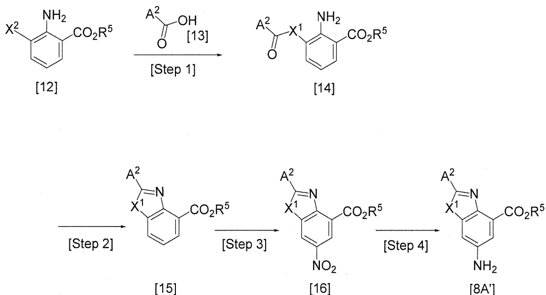
[Formula 7]
