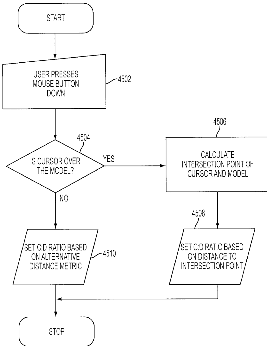
FLOWCHART OF PAN TOOL INITIALIZATION
