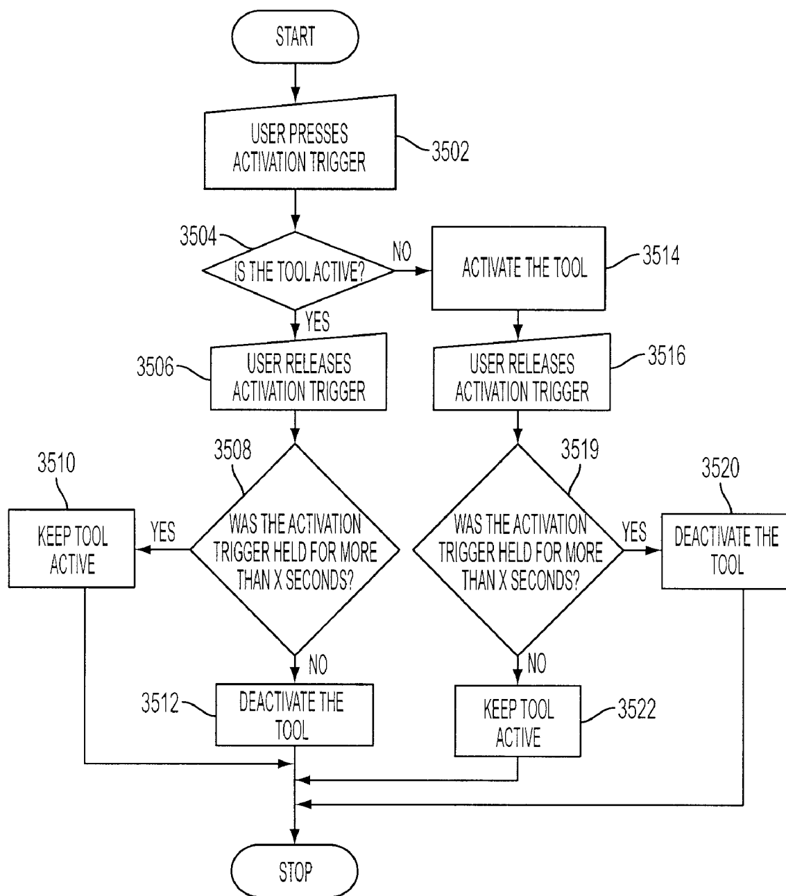
FLOWCHART OF TAP VS. HOLD ACTIVATION
