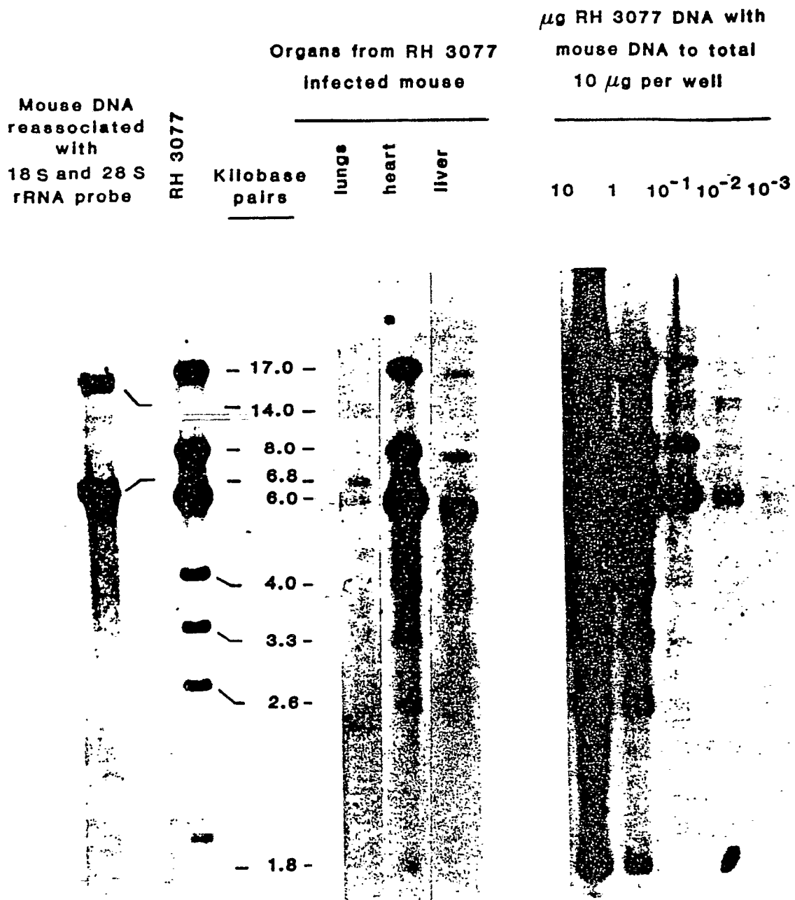
FIG. 12 Detection of S. pneumoniae RH 3077 ribosomal gene sequences in EcoR I digested DNA from infected mouse tissues
