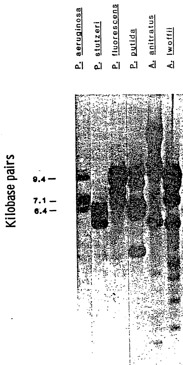
FIG. 4 PST I digested DNA from Pseudomonas and Acinetobacter species
