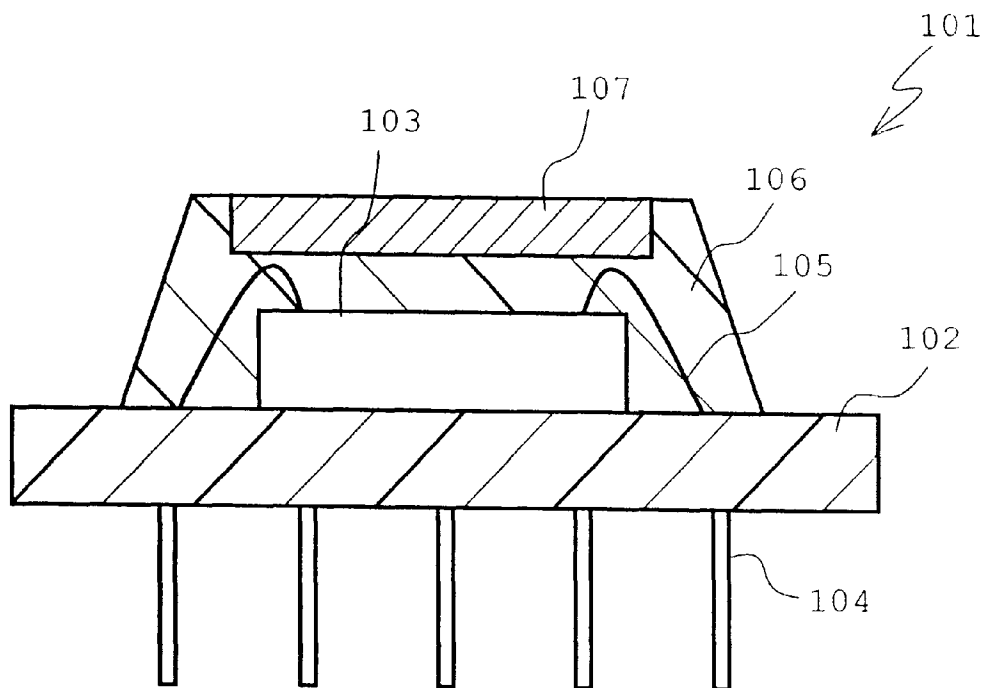
FIG. 7 Prior Art
