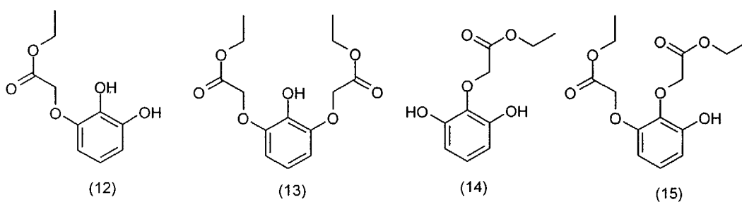
4-Possible alkylated Pyrogallol substructures
