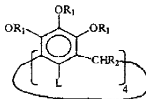
Formel I
