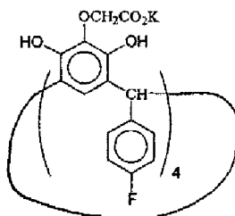
Formel II
