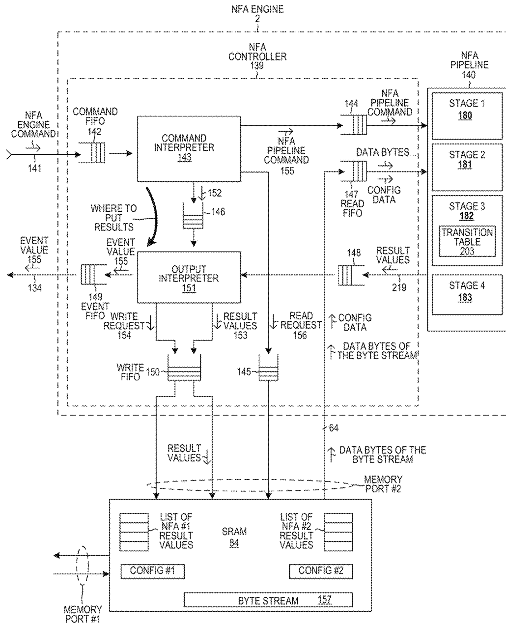
NFA ENGINE AND SRAM FIG. 8
