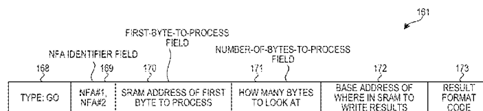
NFA ENGINE GO COMMAND
