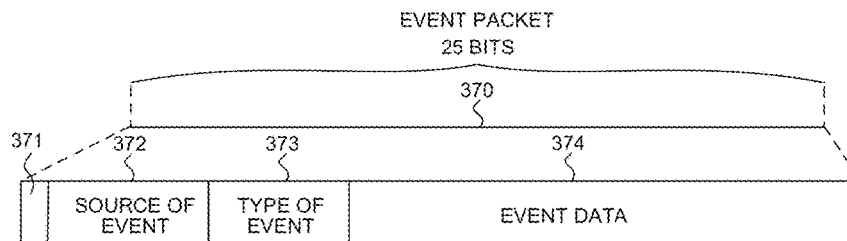
EVENT PACKET BIT SEQUENCE FIG. 30
