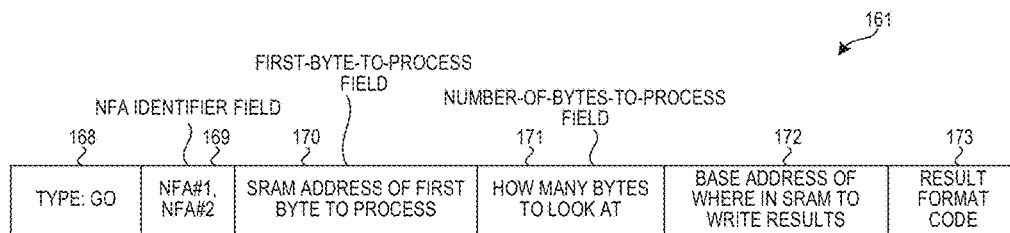
NFA ENGINE GO COMMAND FIG. 10
