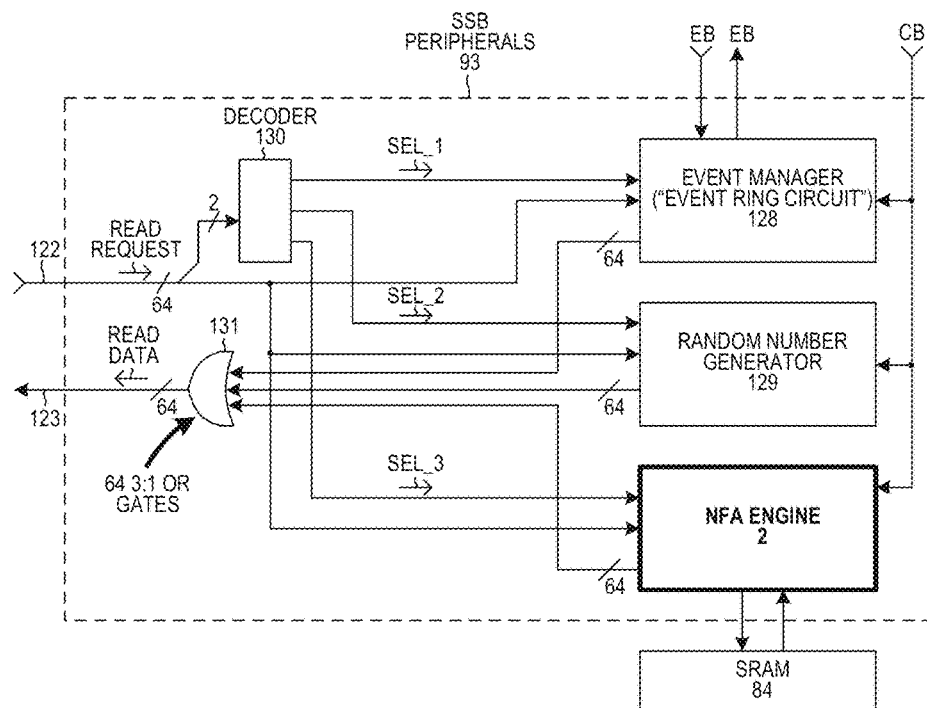
SSB PERIPHERALS BLOCK FIG. 6
