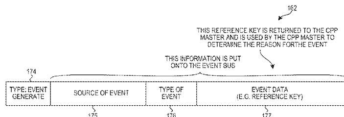
NFA ENGINE EVENT GENERATE COMMAND
