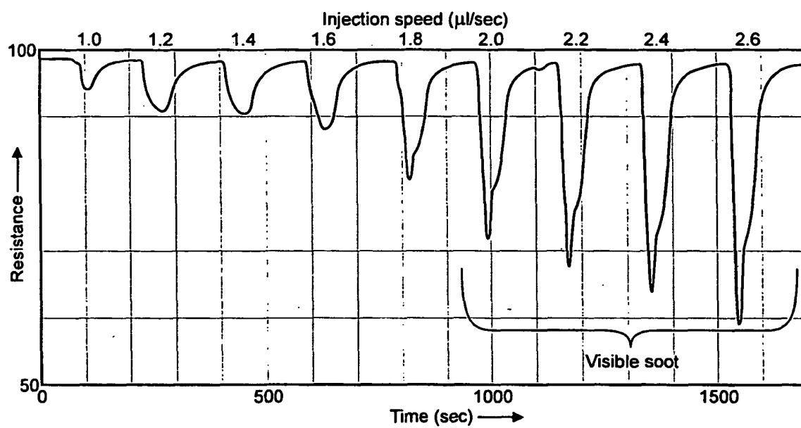
Target gas sensor response with increasing injection speed
