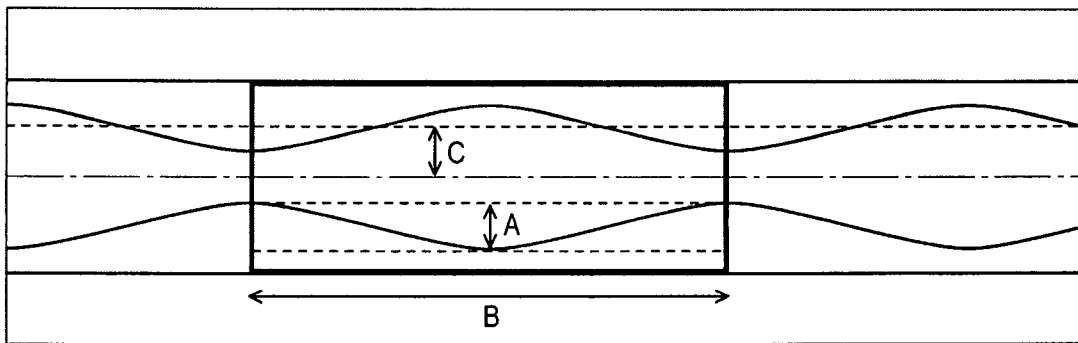
Sinusoid Configuration - Parameters A, B and C
