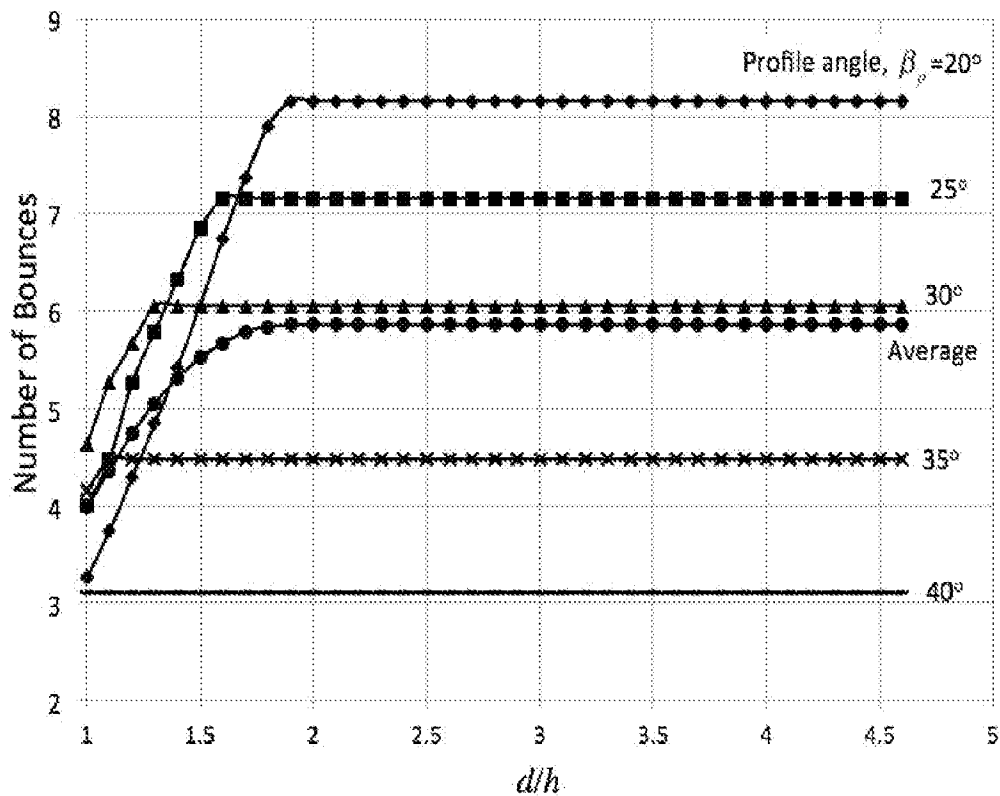
Figure 13: Effect of cavity depth on the number of bounces when cavity surface is 100% specular
