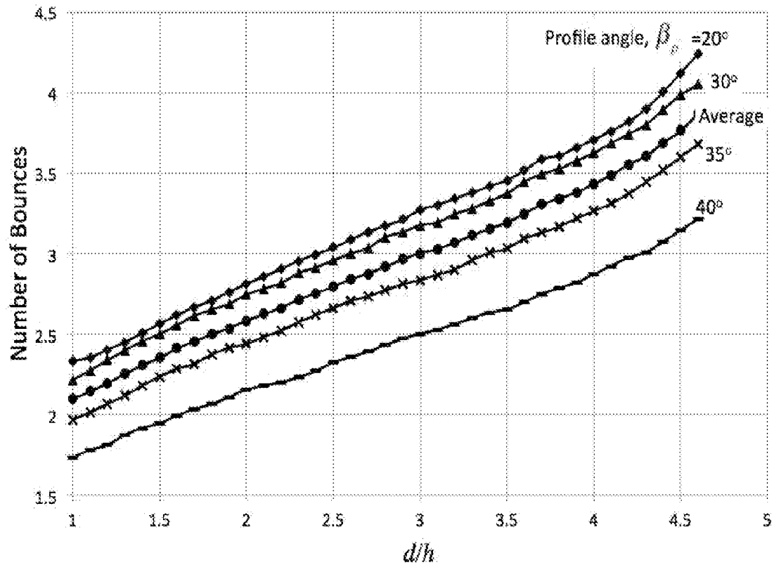
Figure 10: Effect of cavity depth on the number of bounces when cavity surface is 100% diffuse
