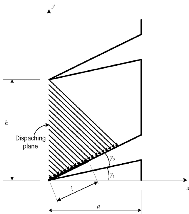
Figure 7: Solar irradiation rays shown with equally spaced rays arriving at a typical cavity groove
