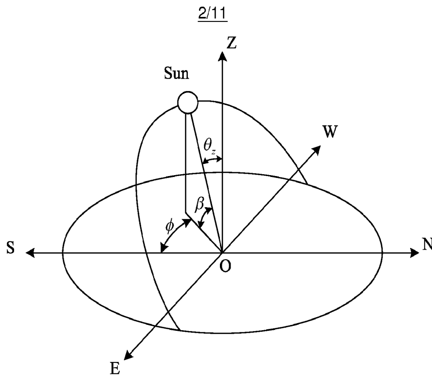
Figure 2: The solar altitude angle \beta , azimuth angle \phi and zenith angle \theta_z
