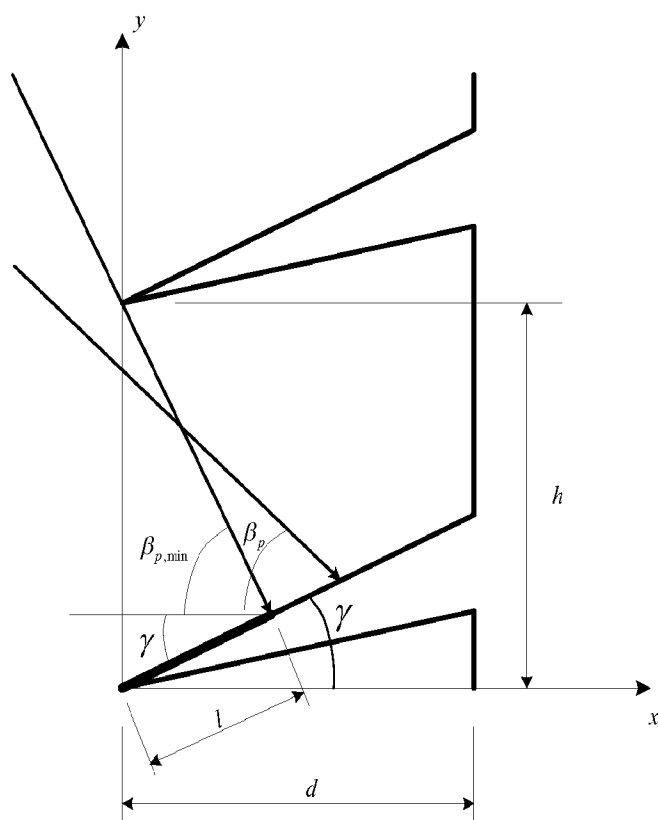
Figure 6: Summer solar ray at minimum projection angle perpendicular to the highly reflective surface
