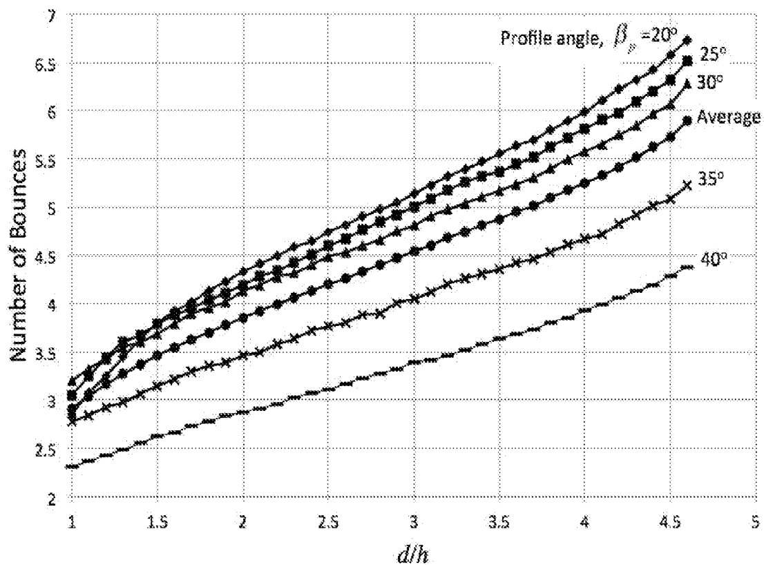
Figure 11: Effect of cavity depth on the number of bounces when cavity surface is 50% diffuse and 50% specular.
