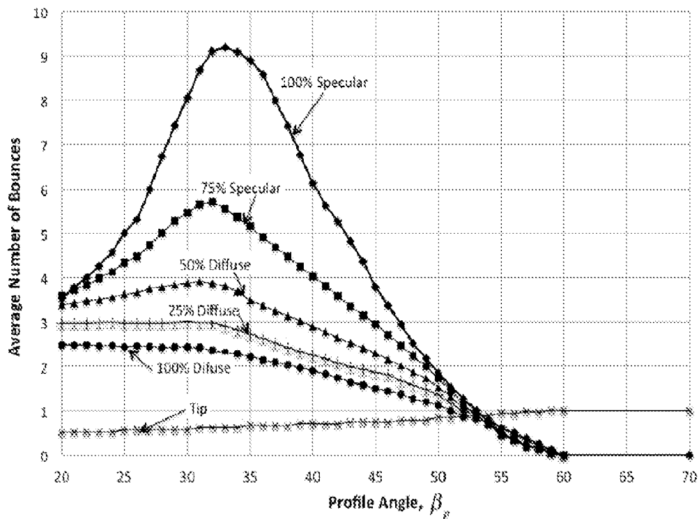
Figure 8: The average number of bounces versus the profile angle for solar rays based on specular, specular-diffuse and diffuse reflections
