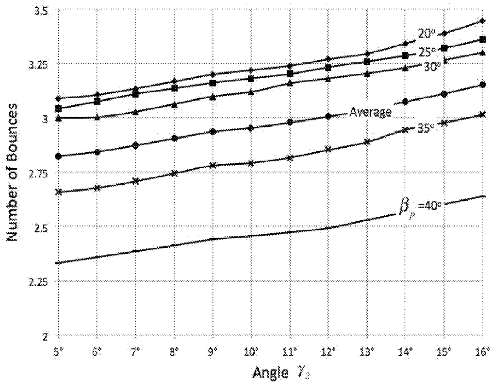
Figure 14: Effect of angle \gamma_2 on the number of bounces when cavity surface is 100% diffuse
