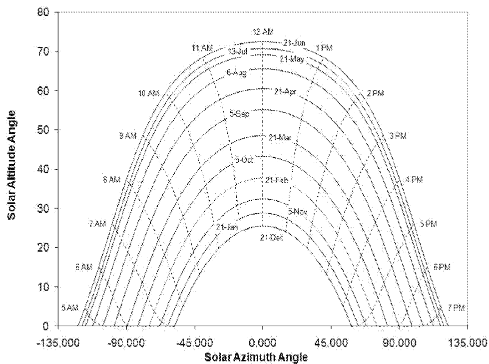
Figure 3: Solar altitude angle versus azimuth angle for latitude of 41^\circ\text{N}
