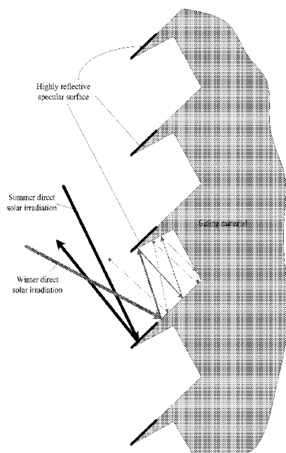
Figure 1: Interaction of summer and winter solar rays with a proposed absorbing/reflecting facade
