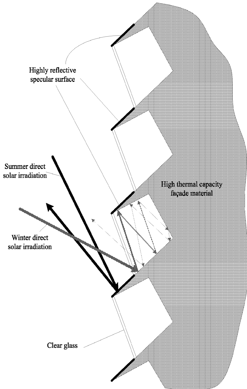
Figure 19: An alternative design with glass-covered cavity
