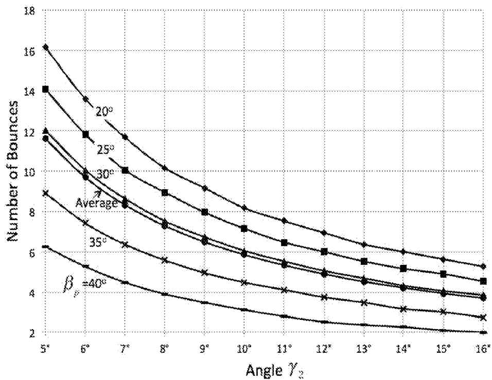
Figure 17: Effect of angle \gamma_2 on the number of bounces when cavity surface is 100% specular
