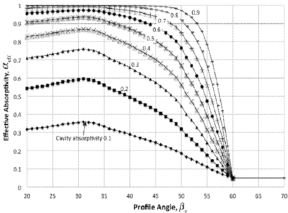
Figure 9: Effective absorptivity versus profile angle for cavity surface absorptivity and tip absorptivity of 0.05.
