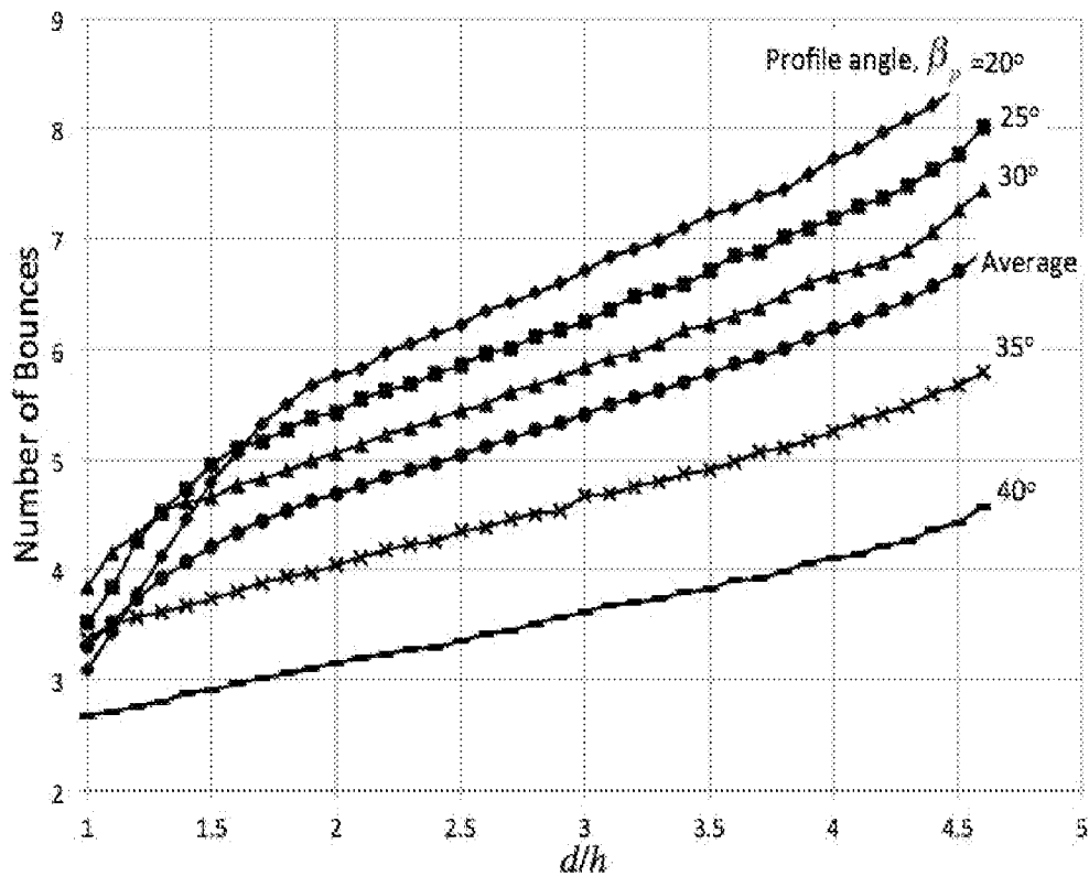
Figure 12: Effect of cavity depth on the number of bounces when cavity surface is 25% diffuse and 75% specular
