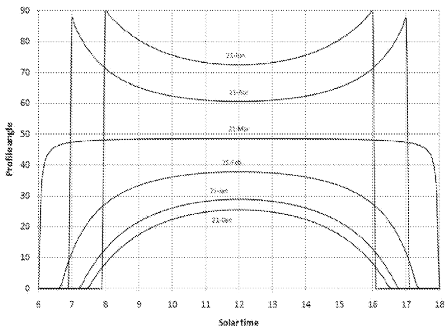
Figure 5: Profile angle for a south facing facade at 41°N
