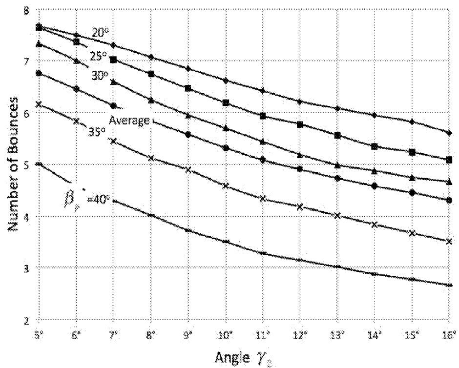
Figure 16: Effect of angle \gamma_2 on the number of bounces when cavity surface is 25% diffuse and 75% specular
