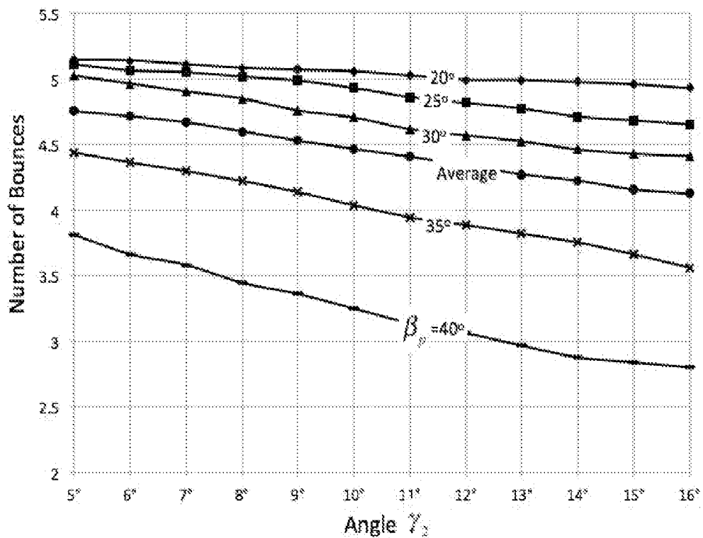
Figure 15: Effect of angle \gamma_2 on the number of bounces when cavity surface is 50% diffuse and 50% specular
