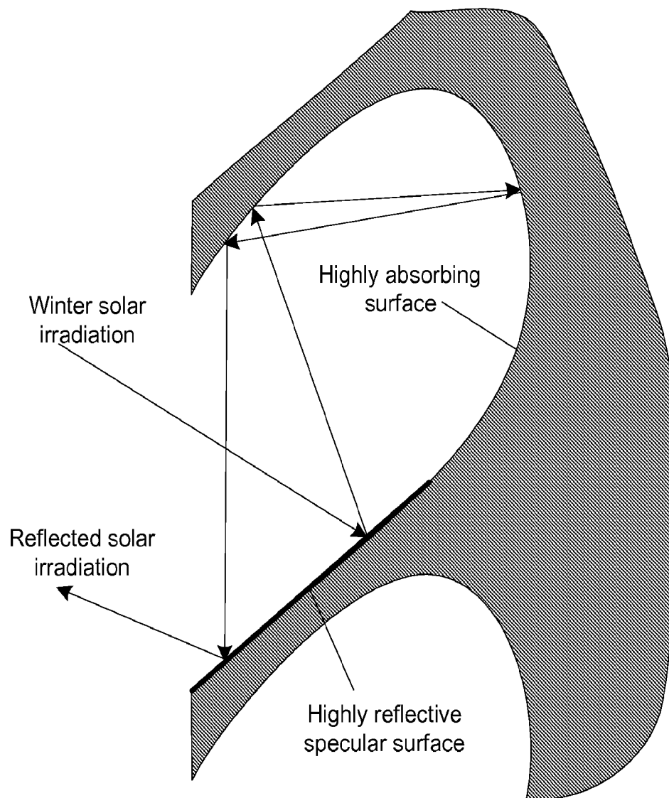
Figure 18: An alternative design with curved cavity surface
