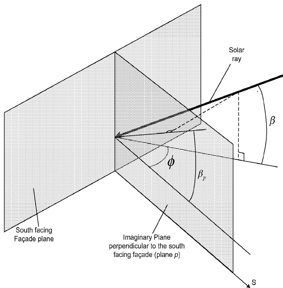
Figure 4: Projection of solar ray on a plane perpendicular to a south facing facade
