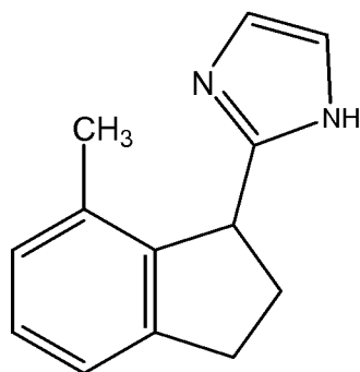
1H-imidazole, 2-(2,3-dihydro-7-methyl-1H-inden-1-yl).
