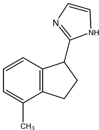
1H-imidazole, 2-(2,3-dihydro-4-methyl-1H-inden-1-yl).
