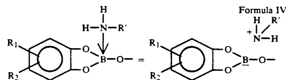
Formula IV illustrates dative bonding.
