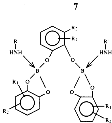
Formula V is a 3:2 catechol to boron complex.
