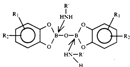
Formula VI is a 1:1 catechol to boron complex.
