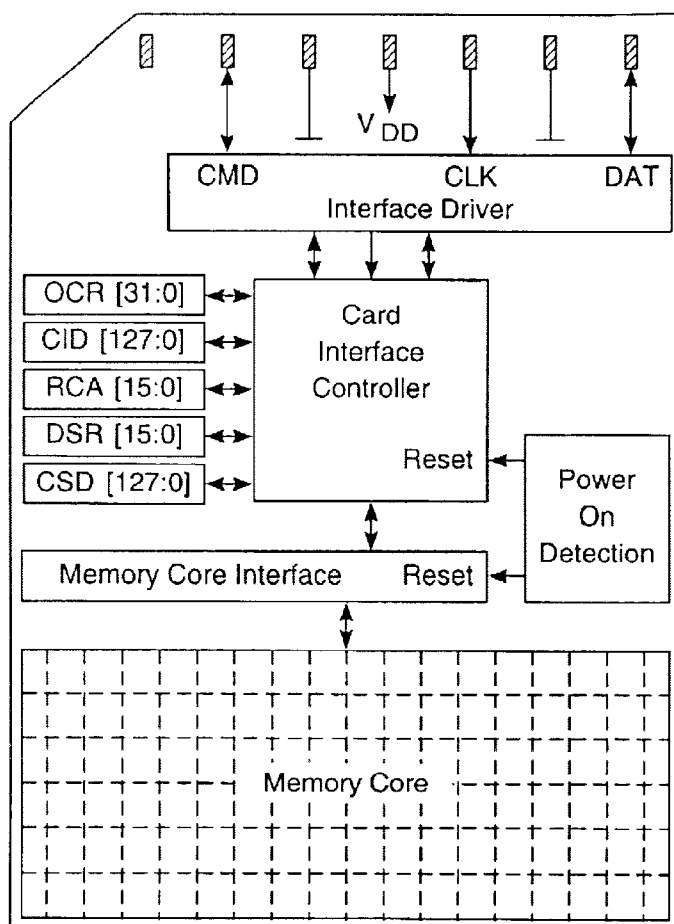
FIG. 6 (PRIOR ART)
