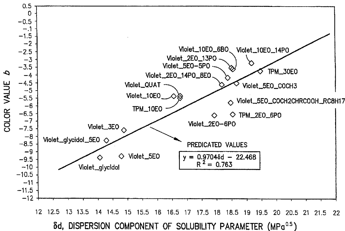
CALCULATED VERSUS MEASURED \delta COLOR VALUES FOR POWDERED CELLULOSE WASHED IN DETERGENT/COLORANT/WATER MIXTURE
