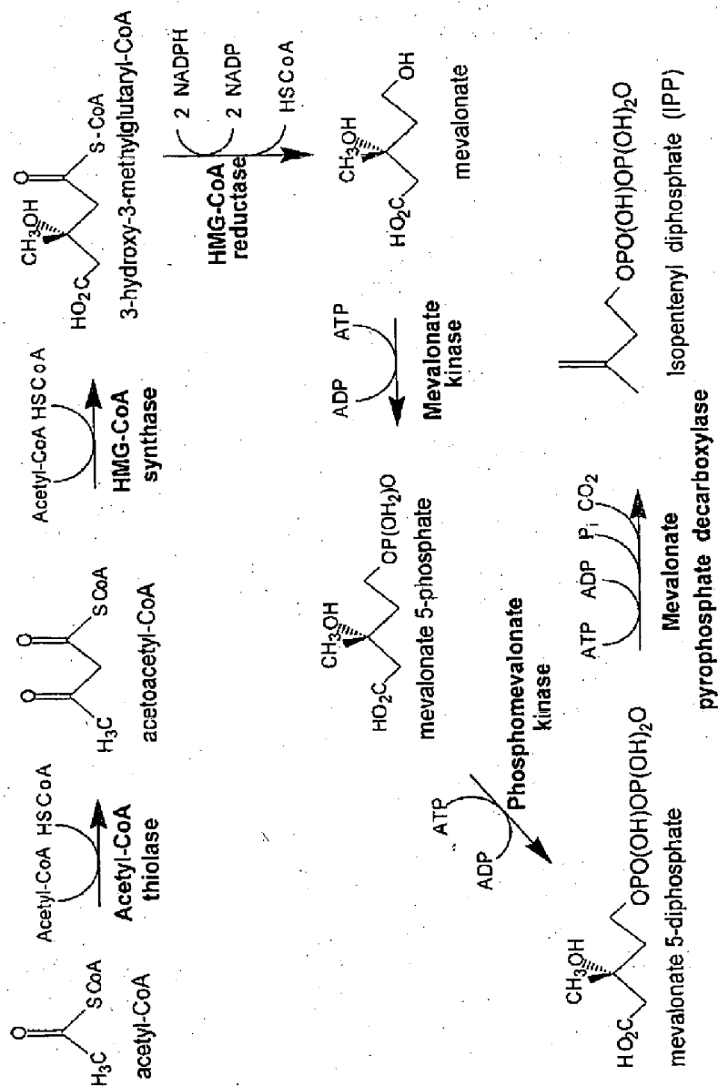
Figure 3 Mevalonate pathway
