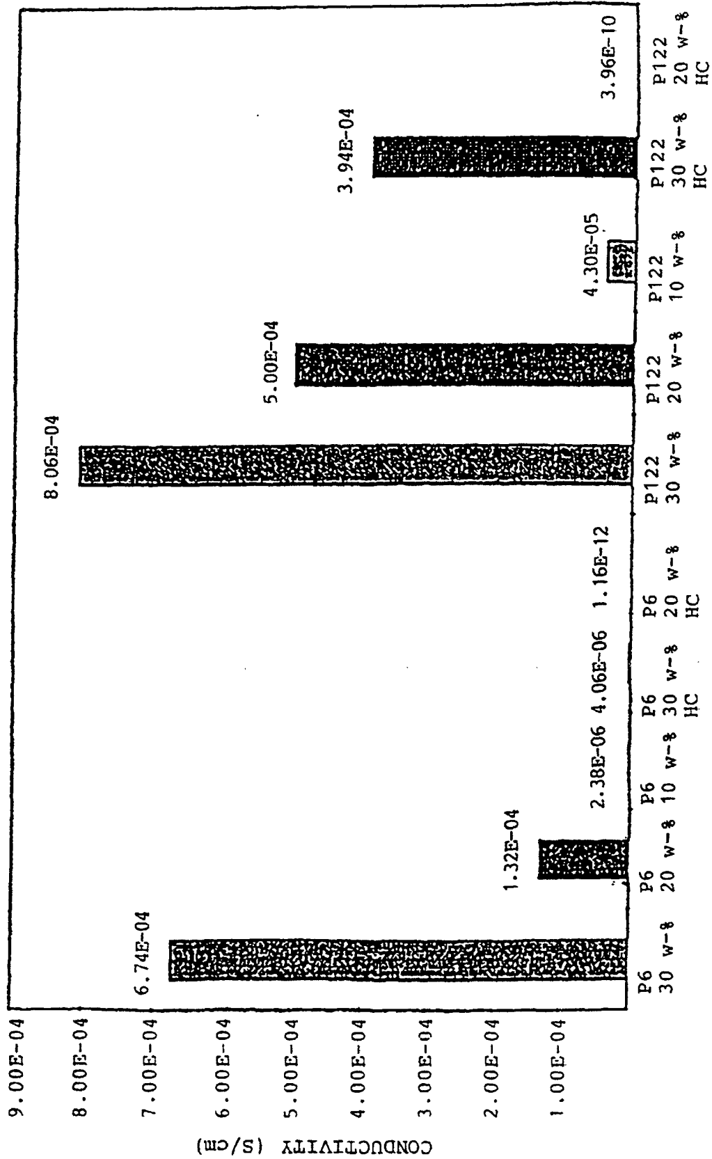
THE CONDUCTIVITY OF PARCEL-ELASTOMERS WITH DIFFERENT PANI-GRADES AND -CONTENTS (150 RPM)
