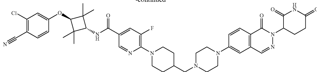
Compound 26
