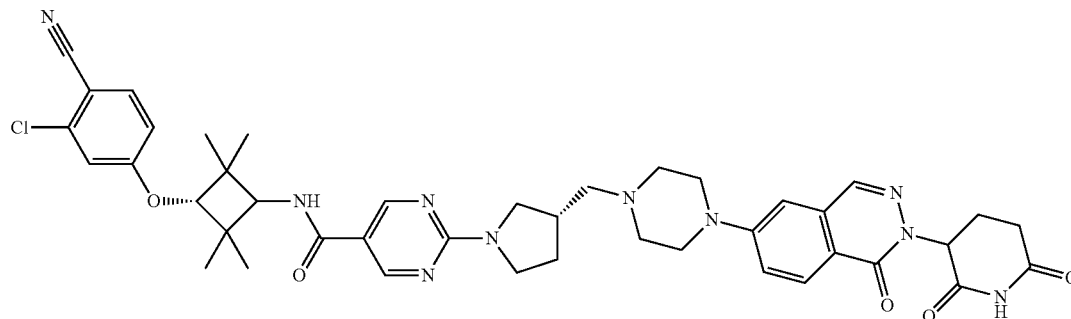
Compound 21
