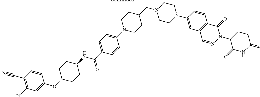
Compound 13
