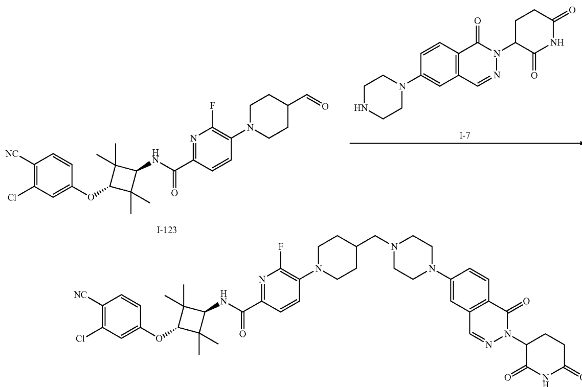
Compound 27
