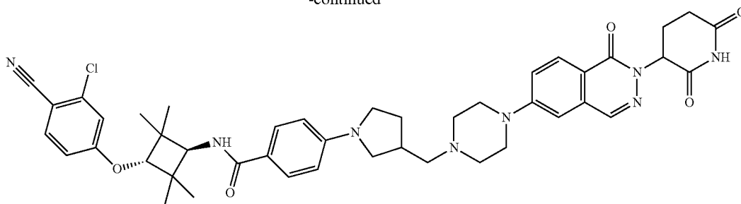
Compound 16
