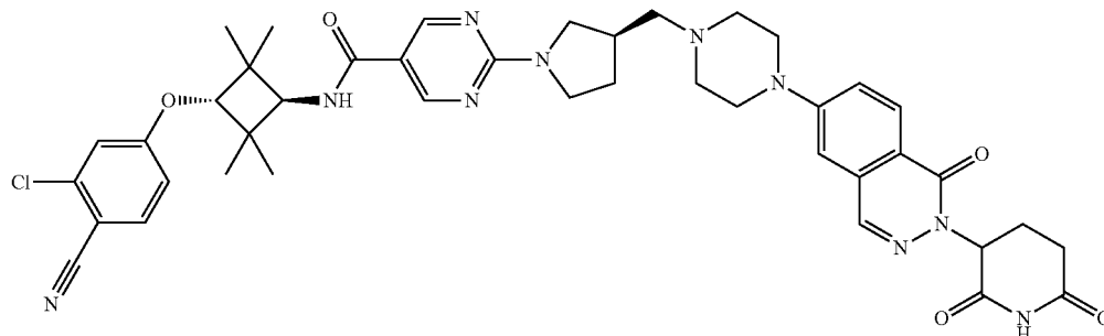
Compound 22
