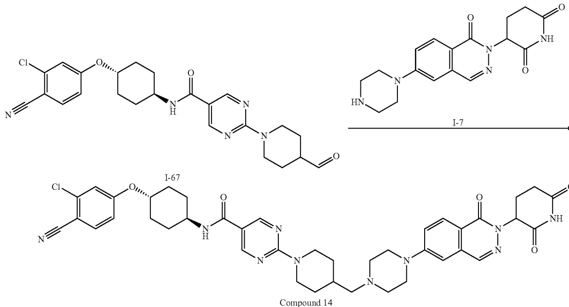
Compound 14
