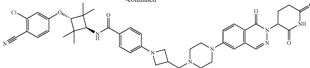
Compound 20
