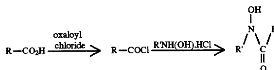
Scheme 3 Preparation of Hydroxyamic Acids
