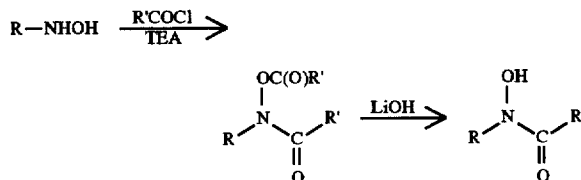
Scheme 4 Preparation of Reverse Hydroxyamic Acids
