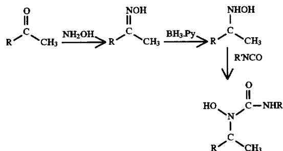
Preparation of Reverse Hydroxyureas
