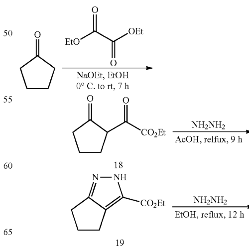
Scheme. Synthesis of UPCDC 864669
