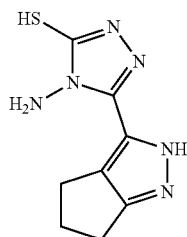
4-Amino-5-(2,4,5,6-tetrahydrocyclopenta[c]pyrazol-3-yl)-4H-1,2,4-triazole-3-thiol (22)
