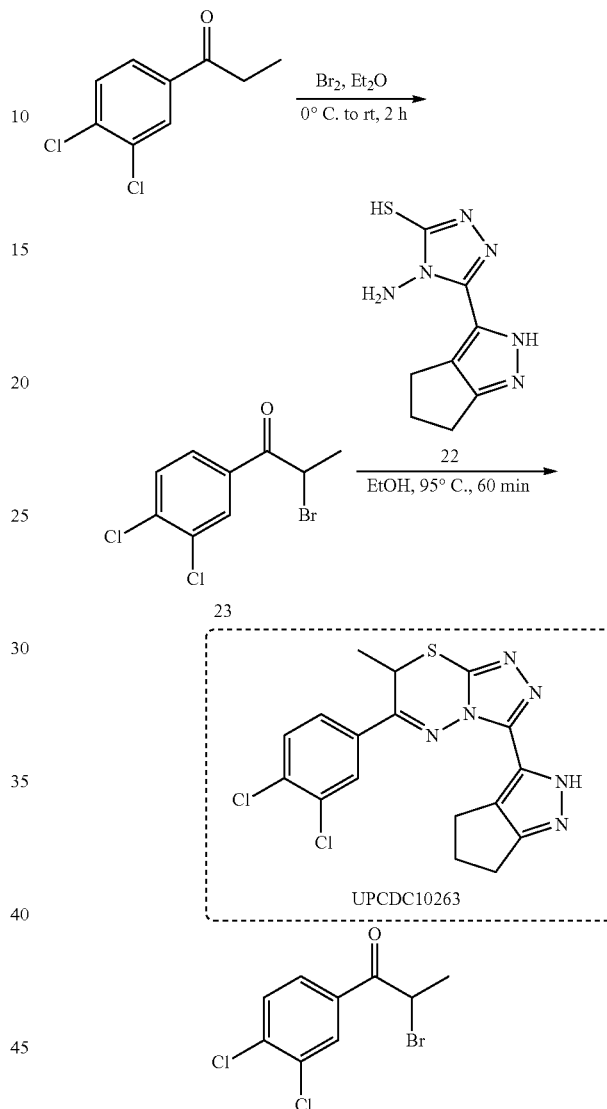
2-Bromo-1-(3,4-dichlorophenyl)propan-1-one (23)
