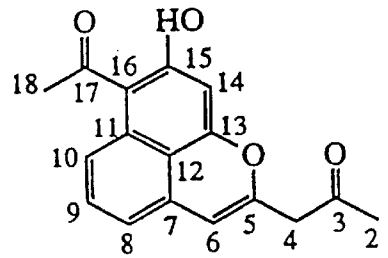
RM 18 (10)
