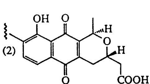
ACTINORHODIN (3)
