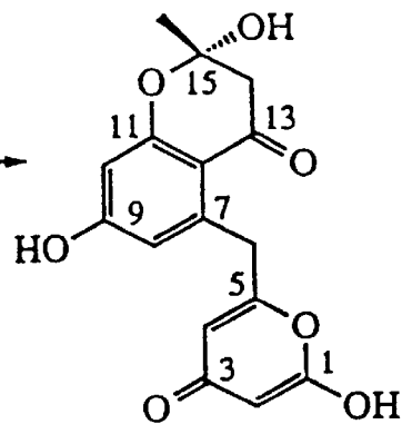
SEK4 (12)
