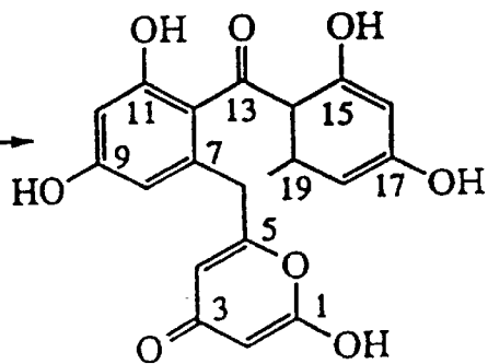
SEK15 (13)
