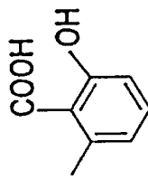
6-METHYLSALICYLIC ACID
