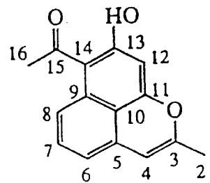
RM 18b (11)
