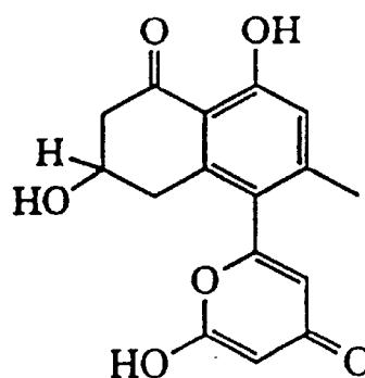
MUTACTIN (6)
