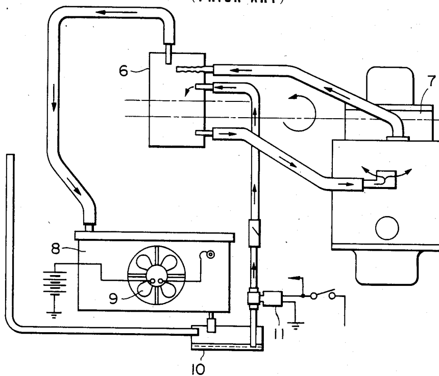
FIG. 3 (PRIOR ART)
