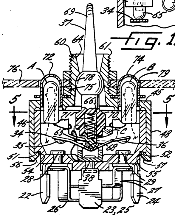
Fig. 3. SWITCH POSITION 2
