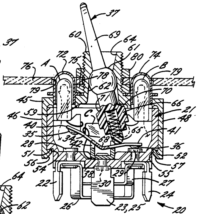
Fig. 2. SWITCH POSITION 1
