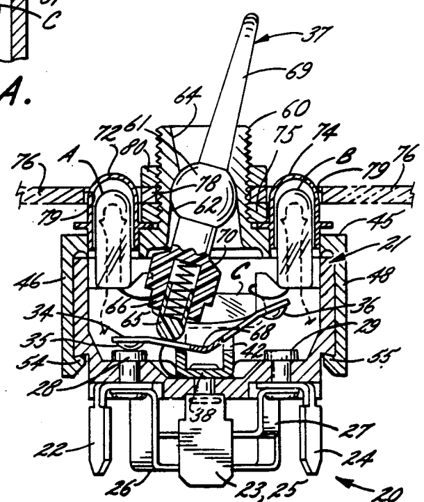
Fig. 4. SWITCH POSITION 3
