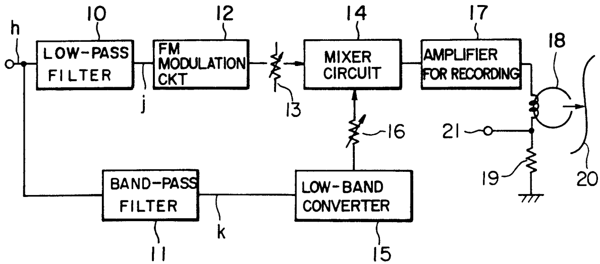
FIG.3 PRIOR ART
