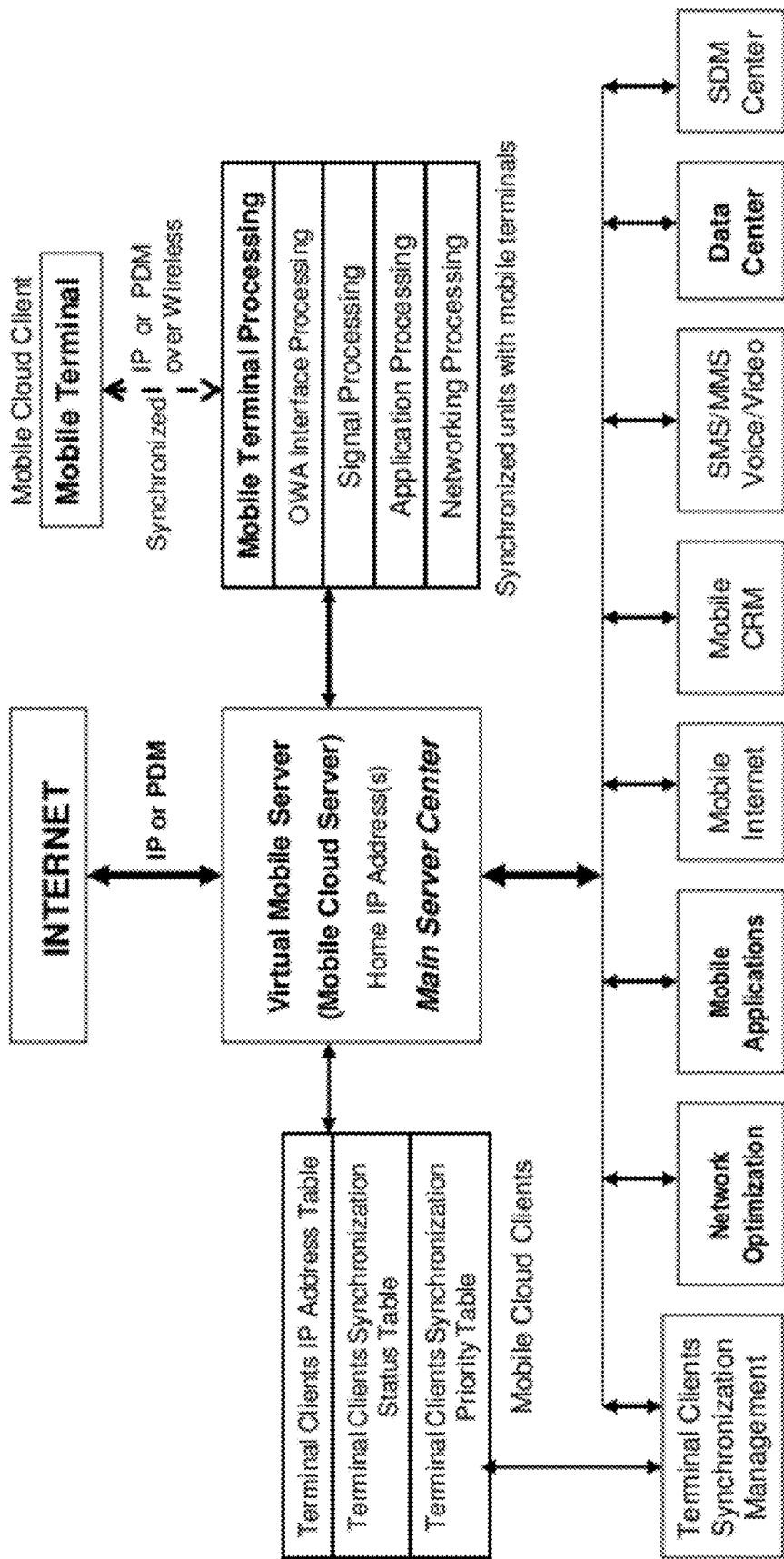
Virtual Mobile Server as Mobile Cloud Server
