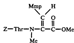
object compound (1)
