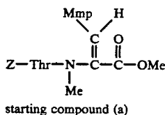
starting compound (a)
