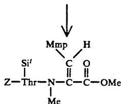
object compound (1)
