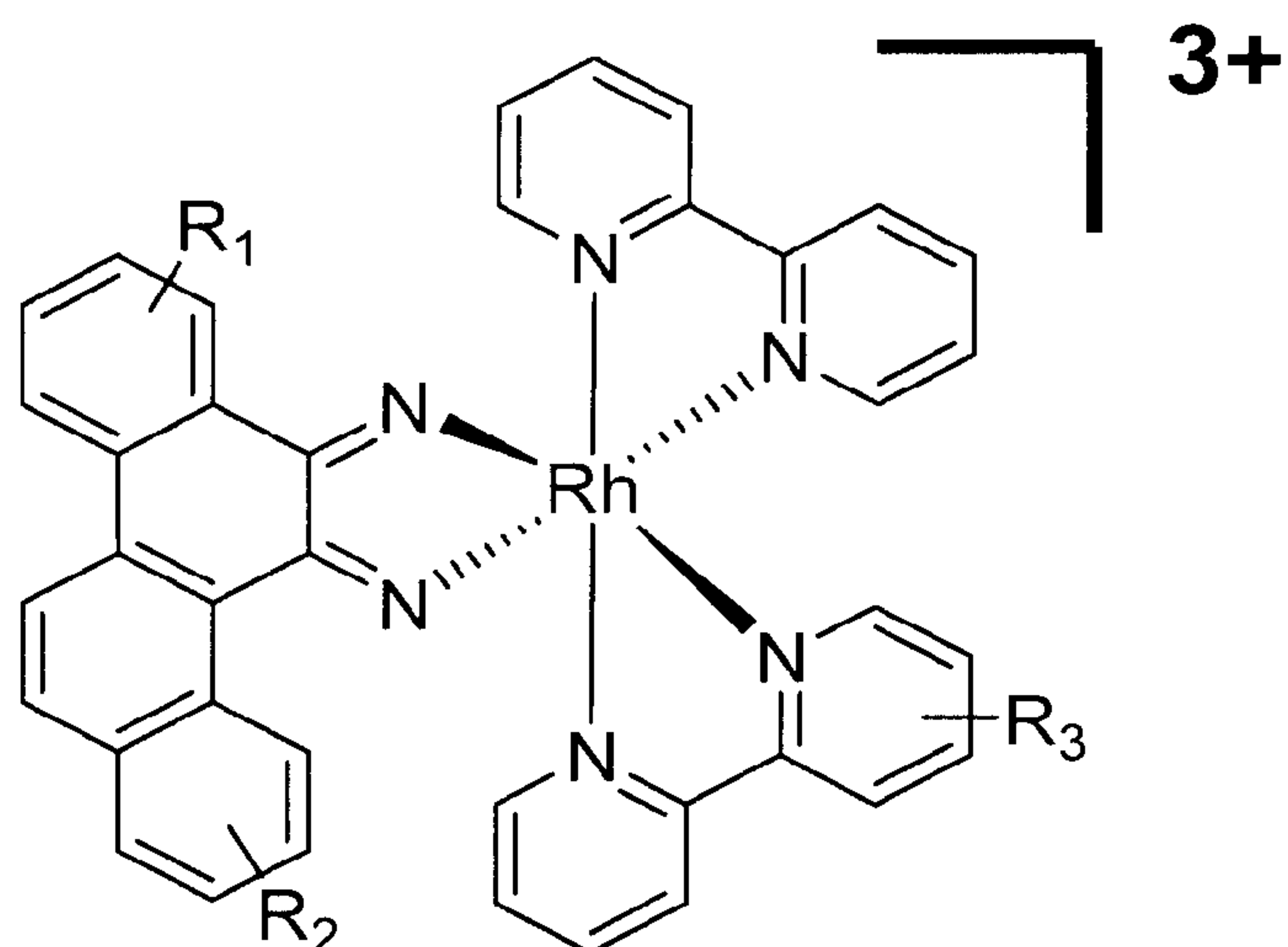
\text{Rh}(\text{bpy})_2(\text{chrysi})^{3+}
