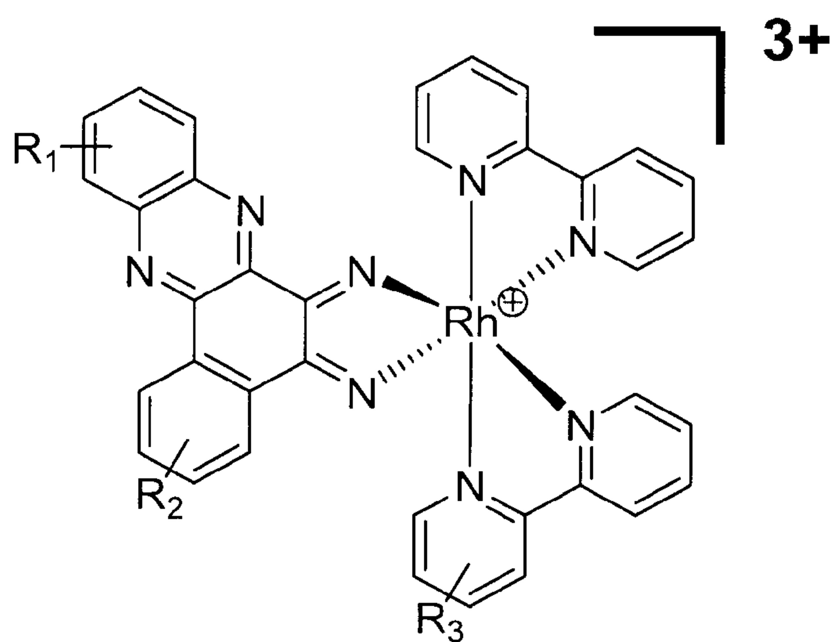
\text{Rh}(\text{bpy})_2(\text{phzi})^{3+}
