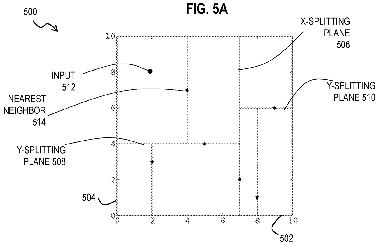
K-D TREE 550
