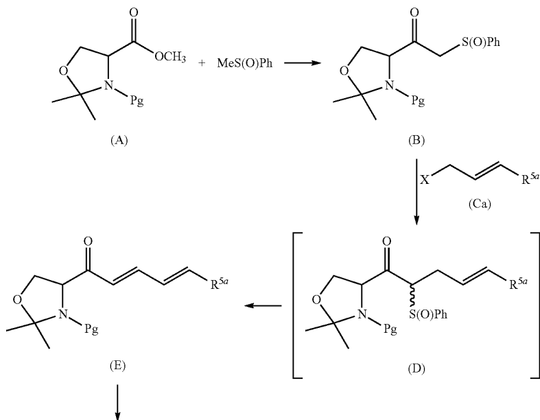
REACTION SCHEME 1
