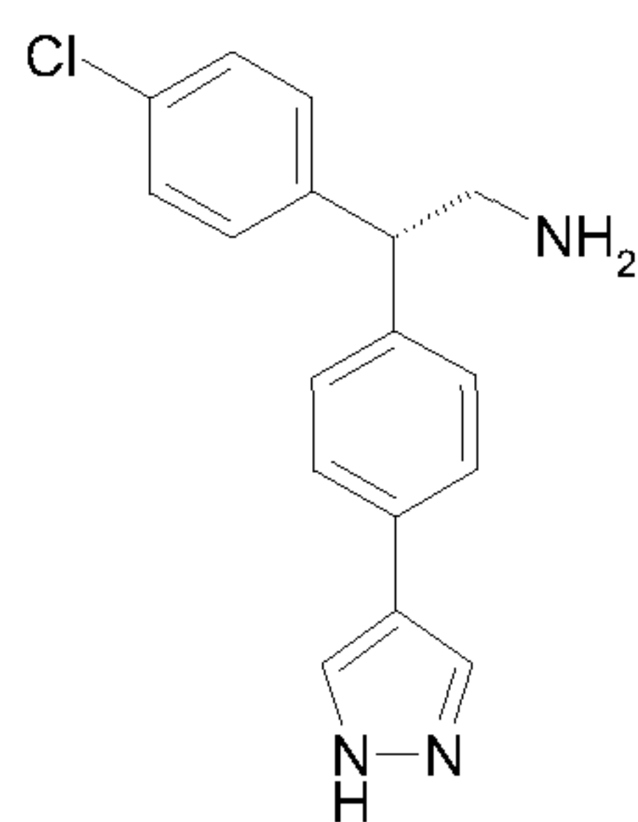
Isomer C
