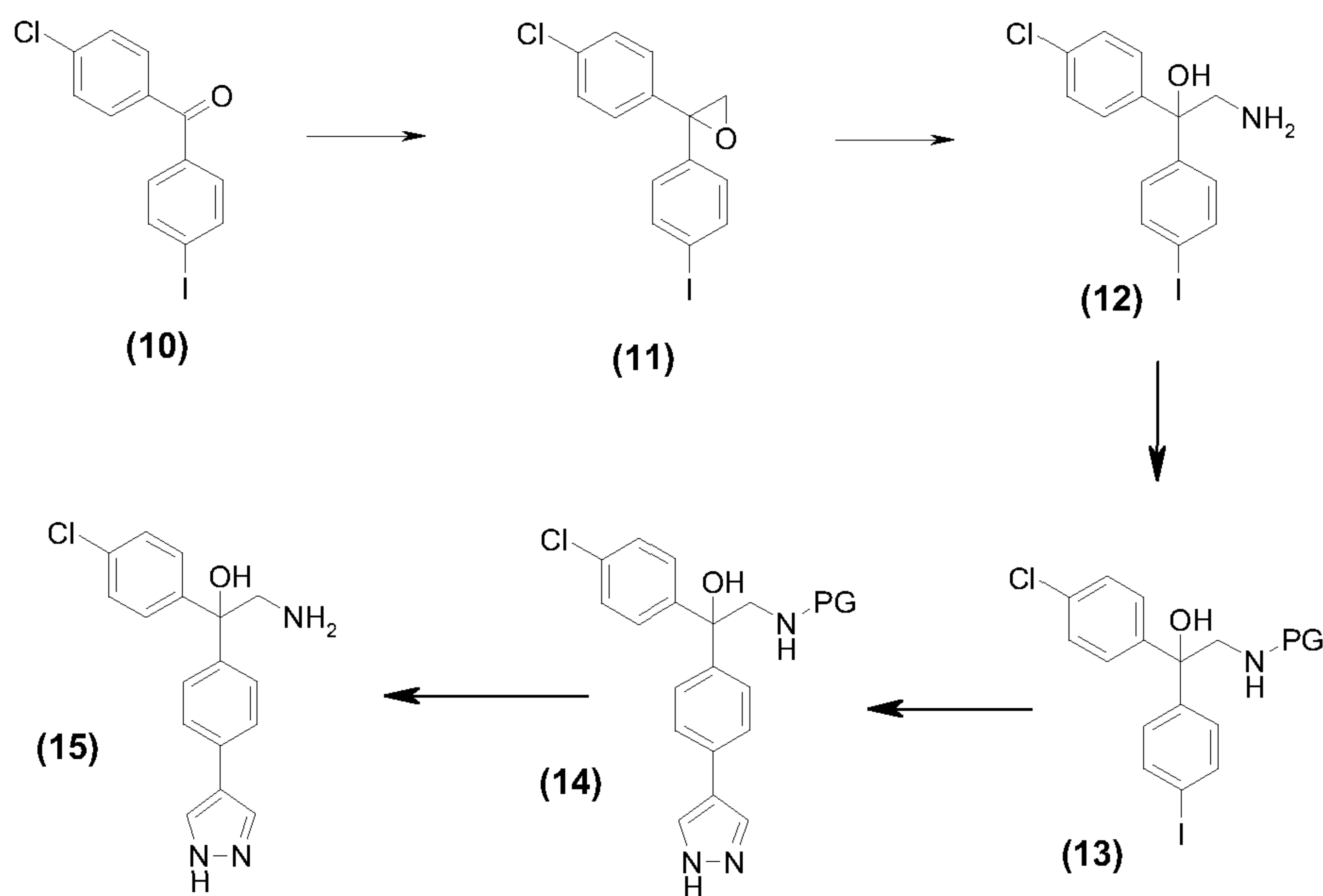
Scheme 1
