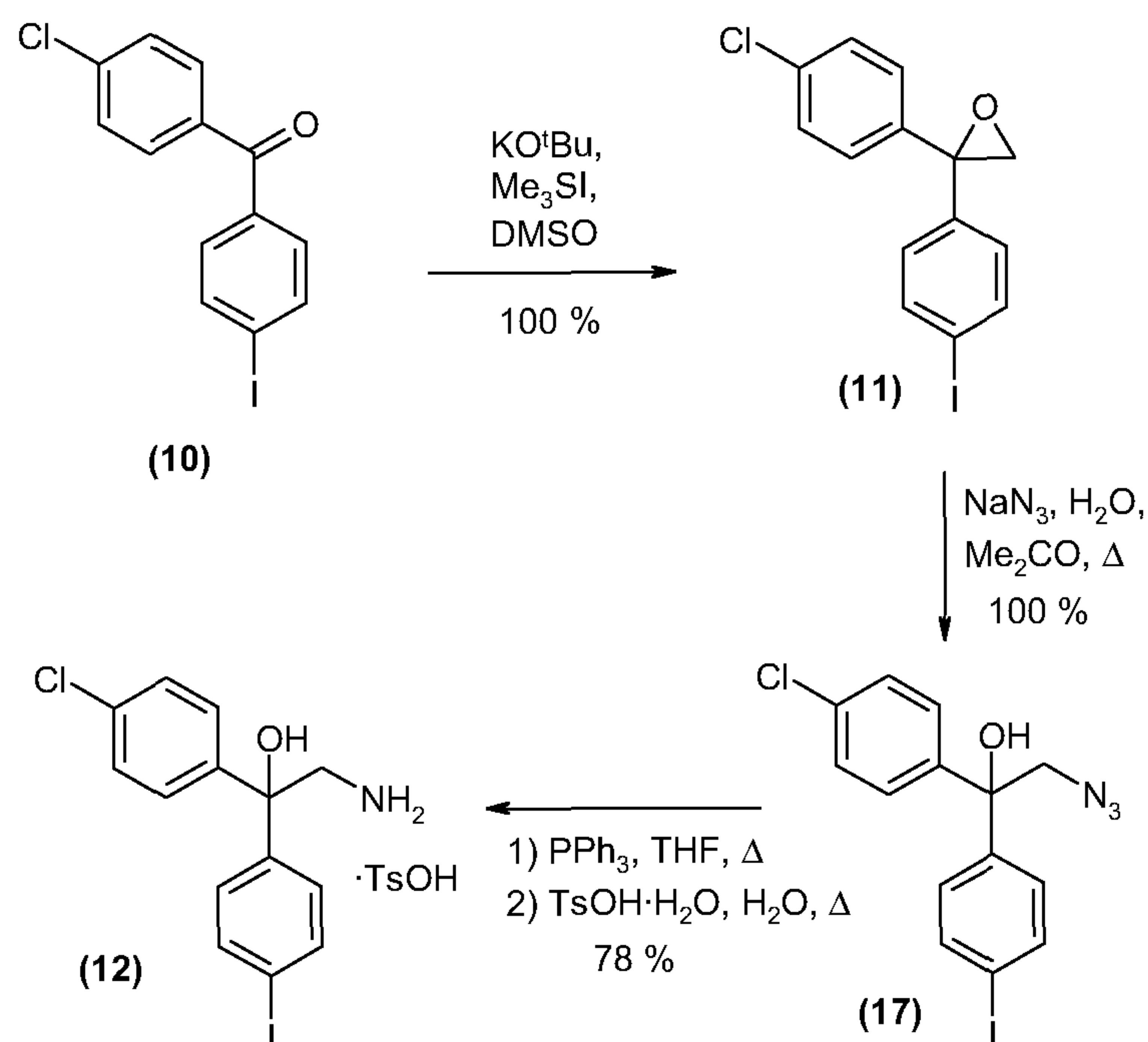
Scheme 2
