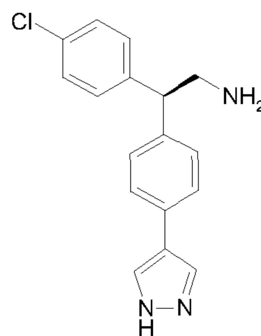
Isomer D
