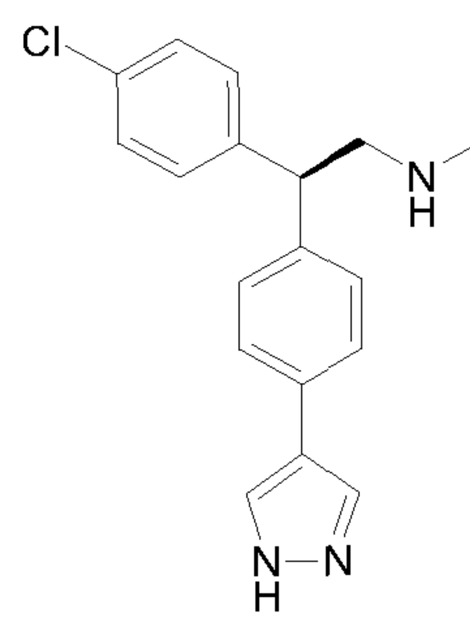
Isomer B
