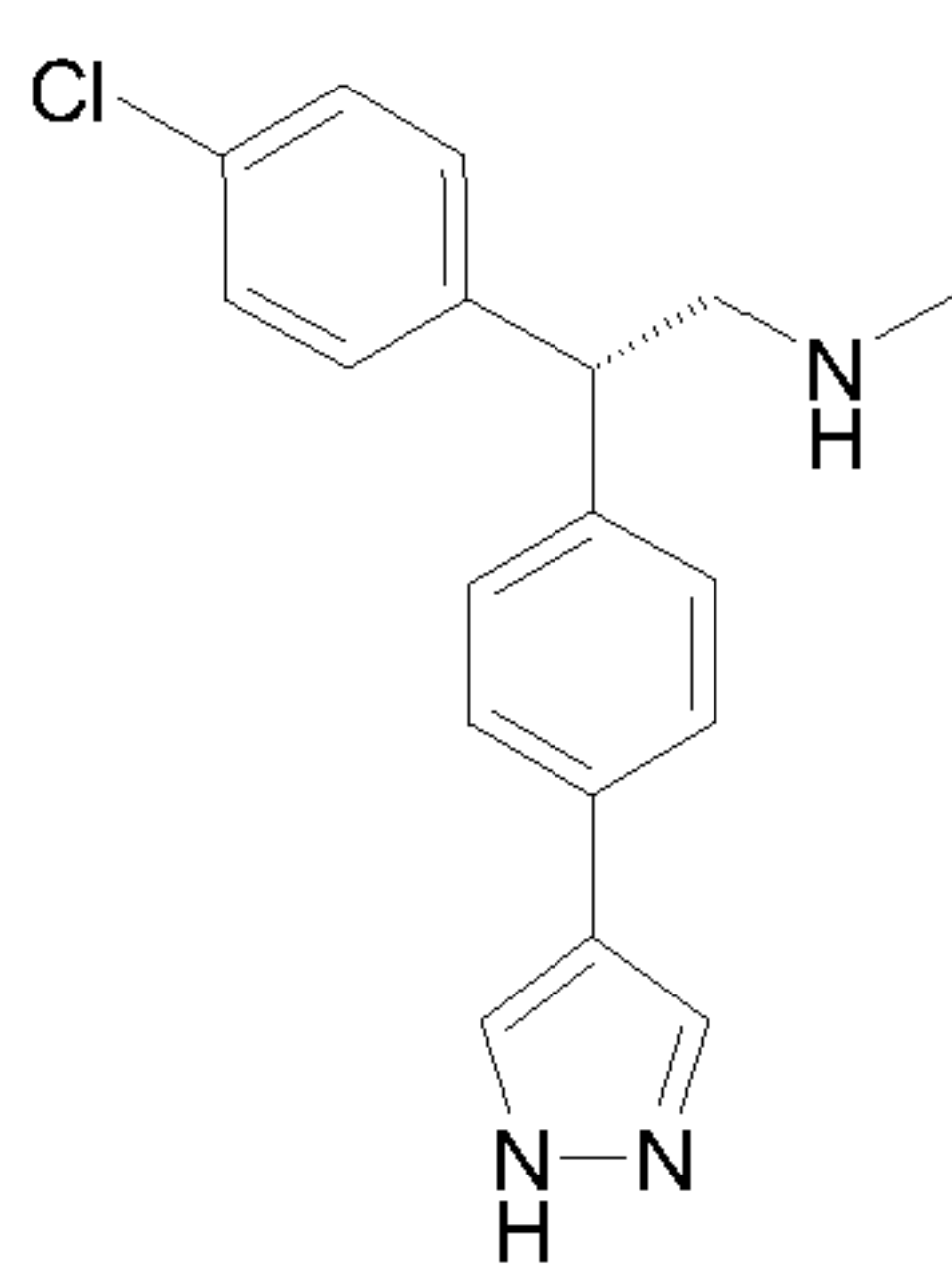
Isomer A
