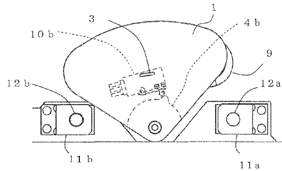
Fig. 6 B Angle of rotation 20^{\circ}
