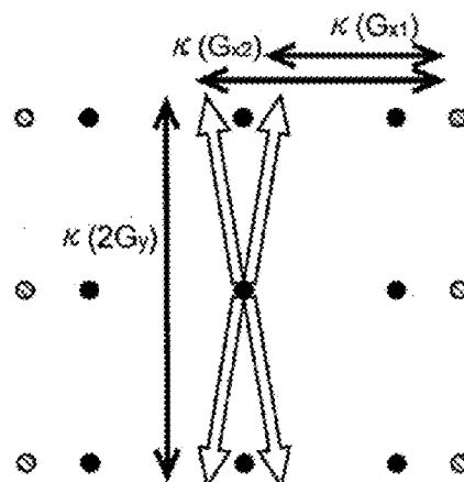
Fig. 5B PRIMITIVE RECTANGULAR (SQUARE) LATTICE + PRIMITIVE RECTANGULAR LATTICE
