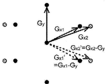
Fig. 4A FIRST RHOMBIC LATTICE + SECOND RHOMBIC LATTICE
