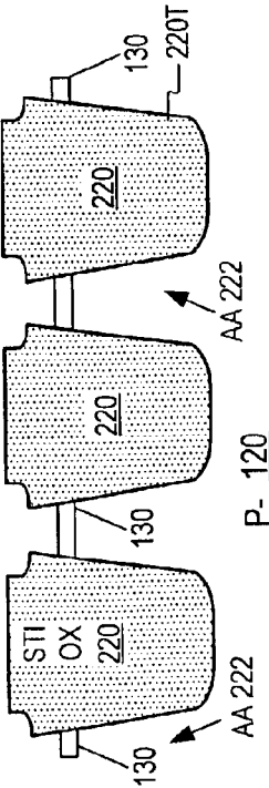
FIG. 5A (Y1-Y1')
