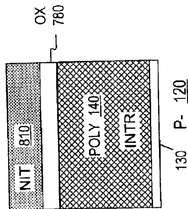
FIG. 19B (PERIPHERY)
