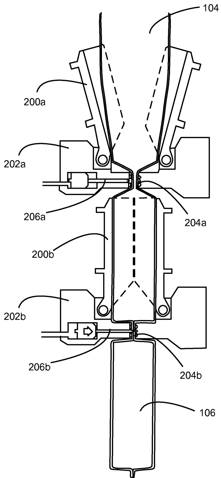
Fig 2 PRIOR ART
