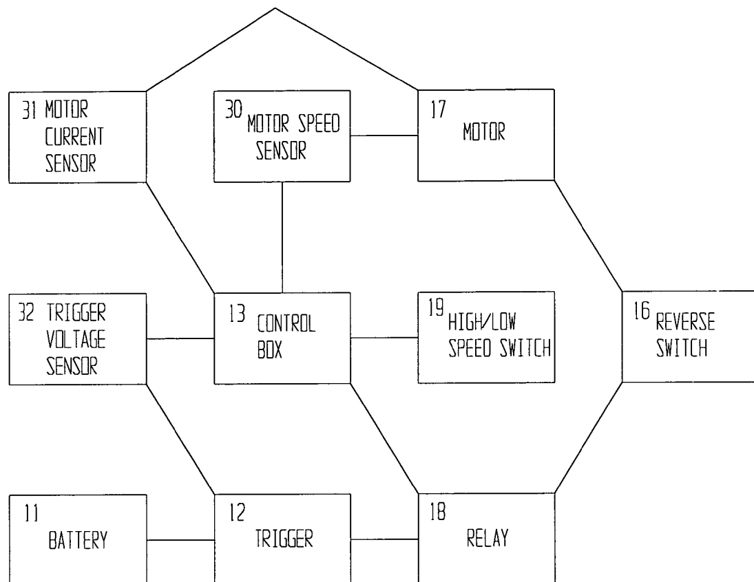
FIG4 AUTOMATIC CONTROLS
