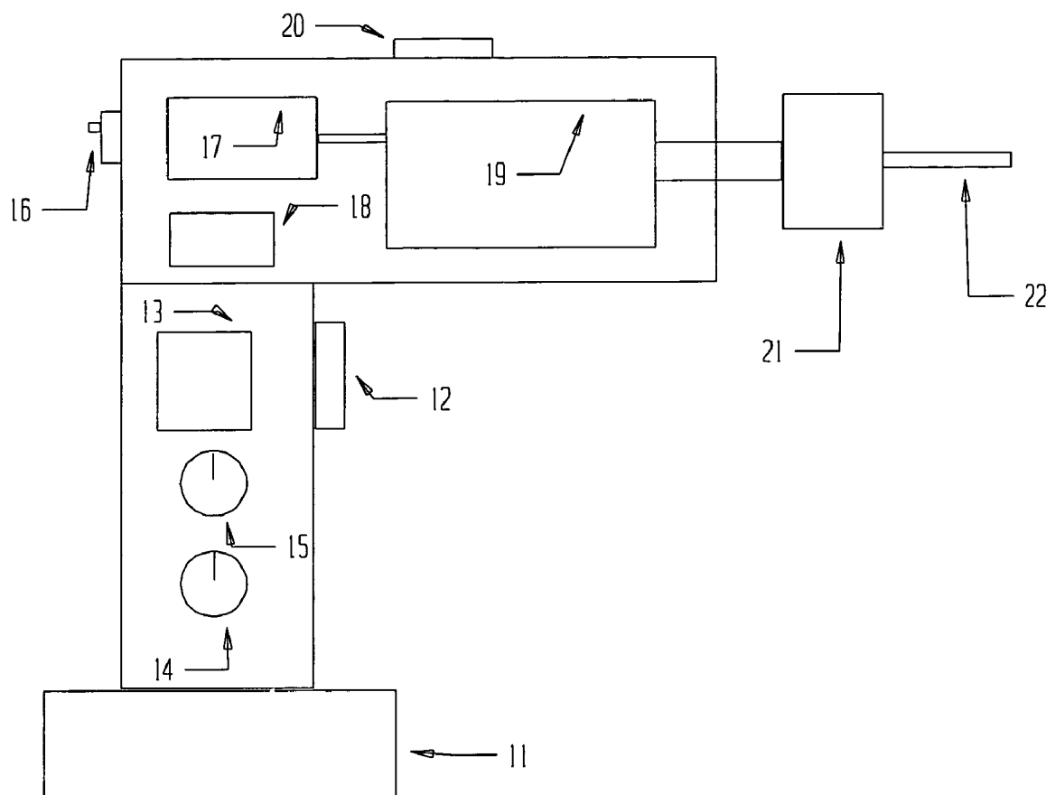
FIG 1 DRILL/DRIVER
