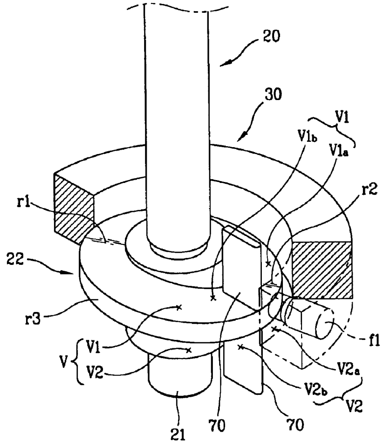
FIG. 4 CONVENTIONAL ART
