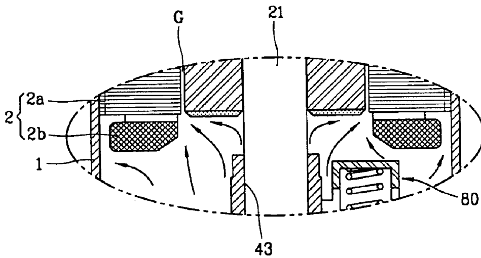
FIG. 4 CONVENTIONAL ART
