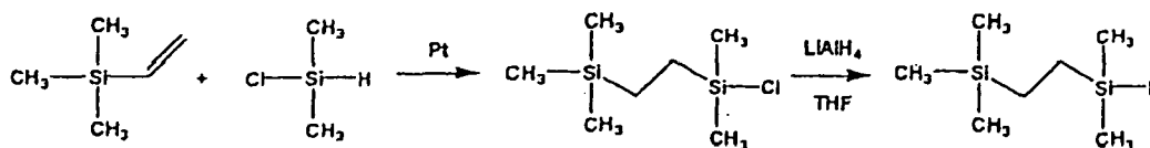
Figure 2 - Reaction Sequence for Preparation of Hydride Intermediate
