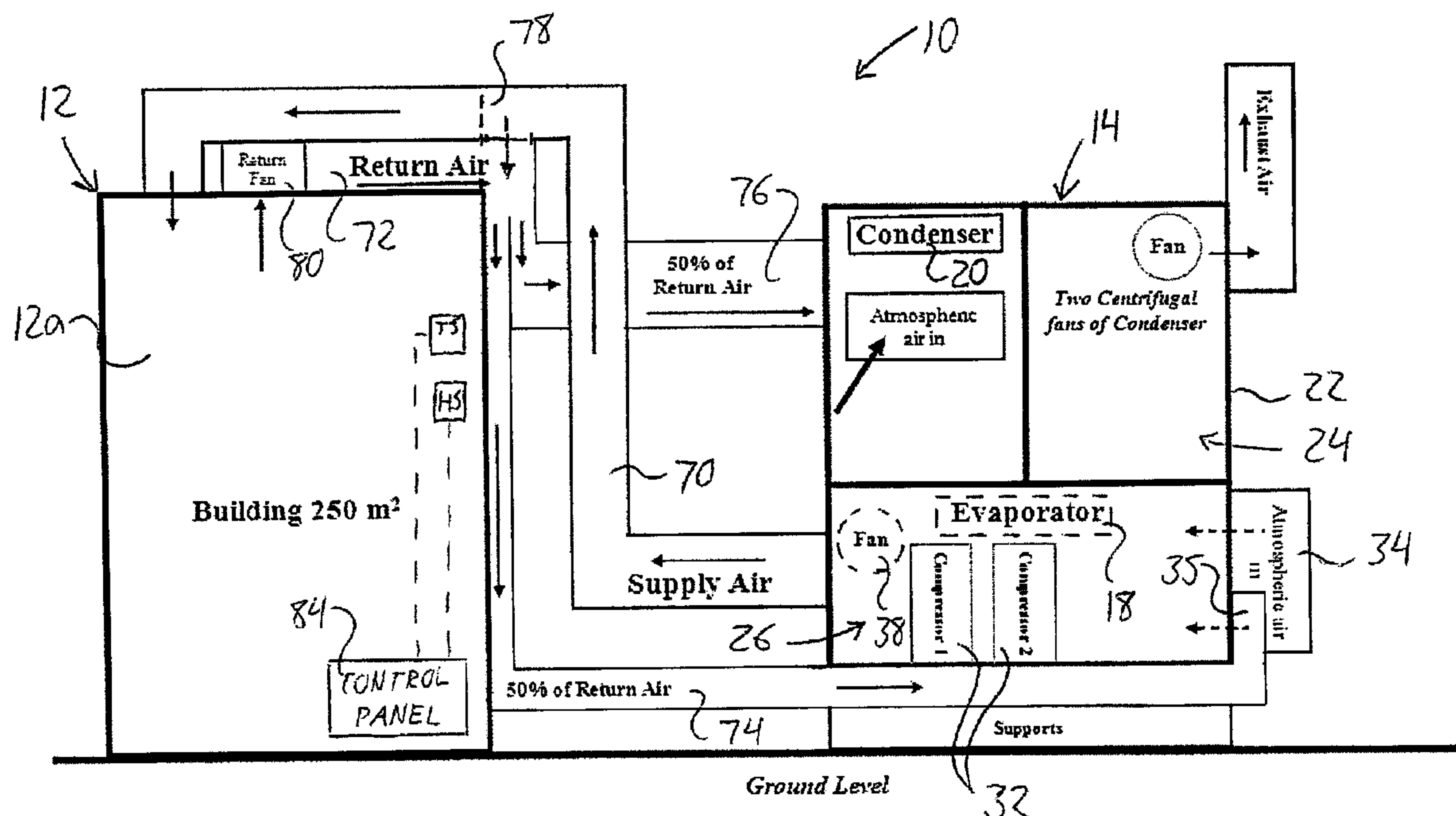
Elevation of the unit (F3) and the building (Not to Scale).
