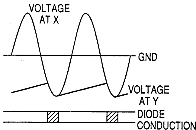
FIG. 2 PRIOR ART
