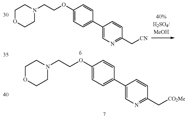
Preparation of methyl 2-(5-(4-(2-morpholinoethoxy)phenyl)pyridin-2-yl)acetate (7)
