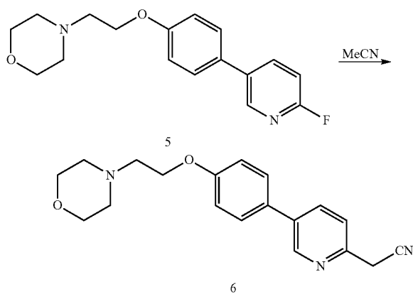
Preparation of 2-(5-(4-(2-morpholinoethoxy)phenyl)pyridin-2-yl)acetate (6)
