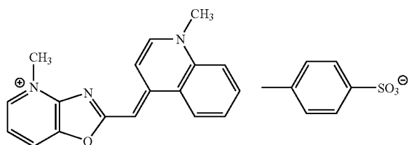
Compound 14
