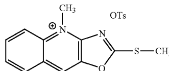
4-methyl-2-methylthioxazolo[4,5-b]quinolinium tosylate
