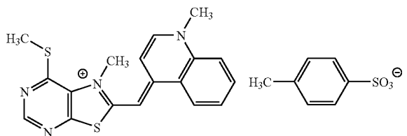
Compound 36
