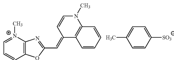
Compound 48
