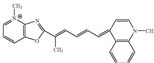
Compound 59
