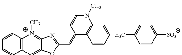
Compound 37
