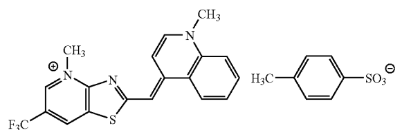
Compound 38
