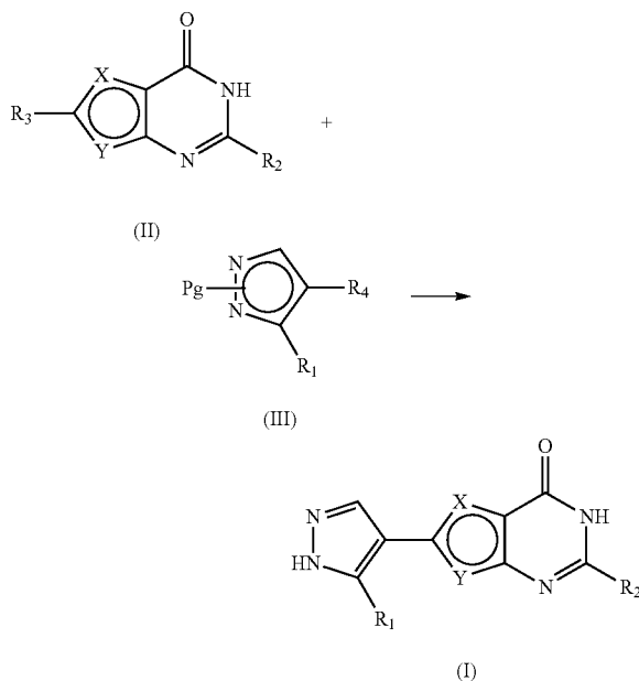
(Reaction scheme 1)
