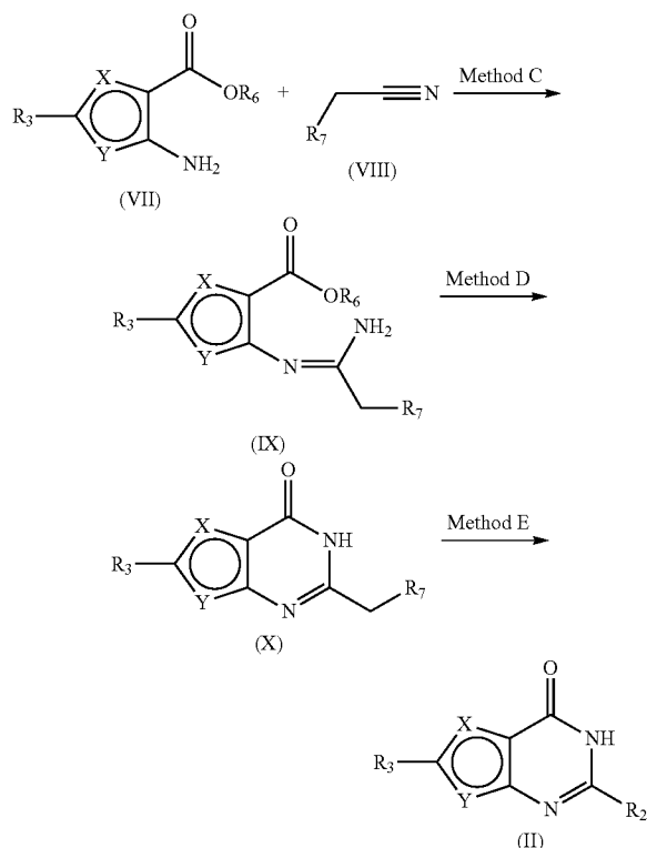
(Reaction scheme 3)
