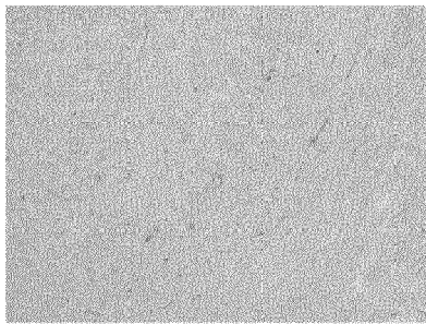
Maleic Acid + dH2O
