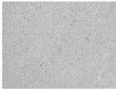
Maleic Acid + Guanidine
