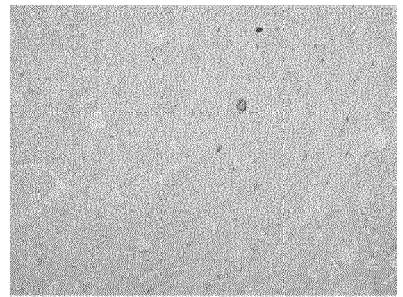
Maleic Acid + 2,2,2- Trifluoroethanol
