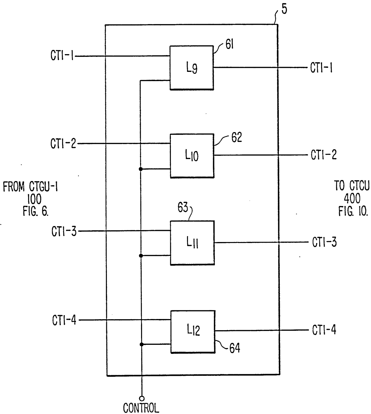
FIG. 8. CTGU-1 REGISTER
