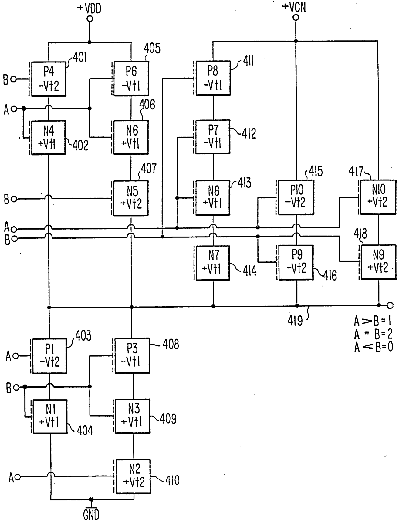
FIG. 10A. TRINARY LOGIC COMPARATOR
