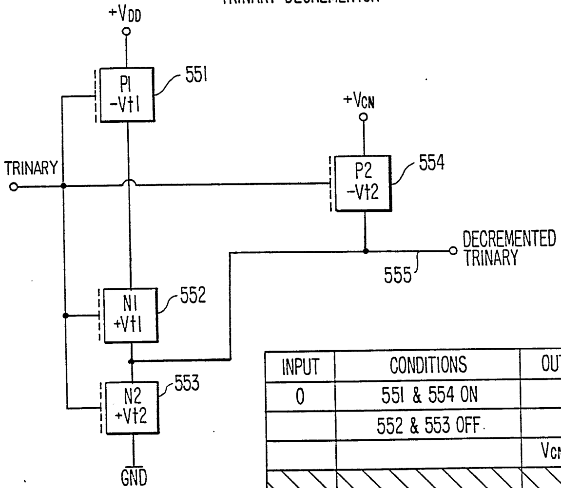
TRINARY DECREMENTOR
