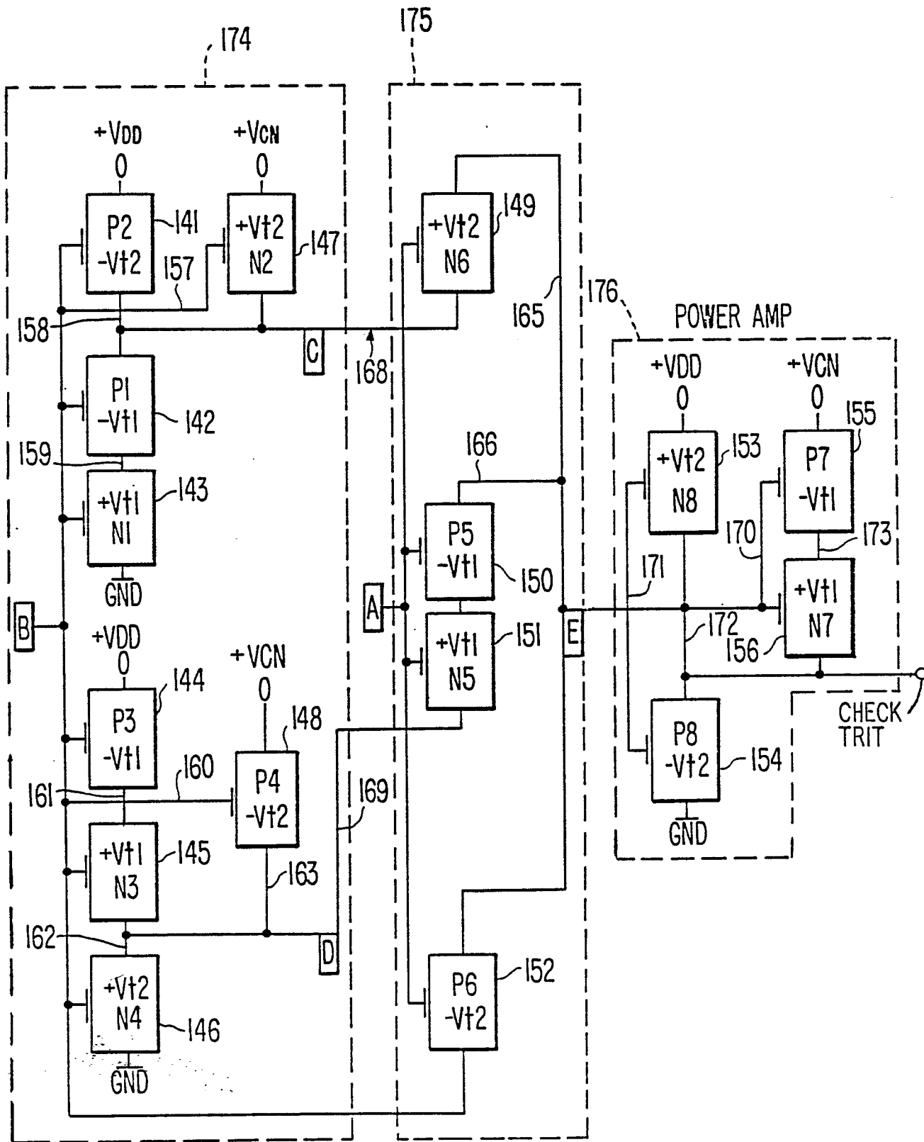
FIG. 3. TRINARY CHECK TRIT GENERATOR
