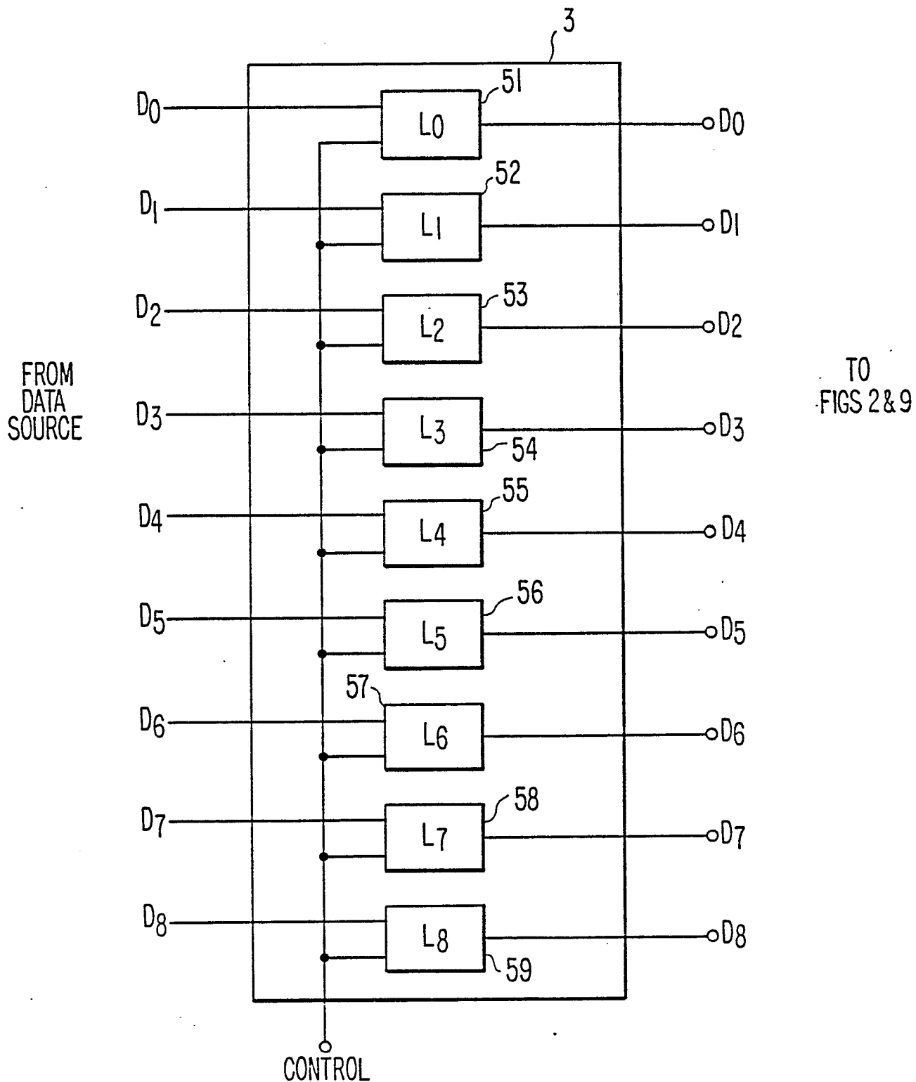
FIG. 7 CTGU-2 REGISTER
