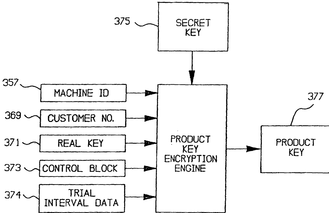
GENERATION OF PRODUCT KEY FIG. 14
