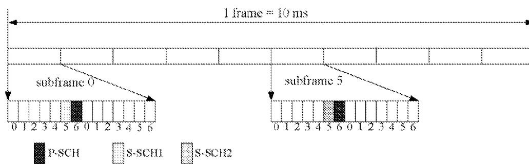
(a) FDD frame structure mode
