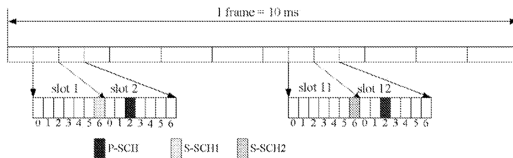
(b) TDD frame structure mode
